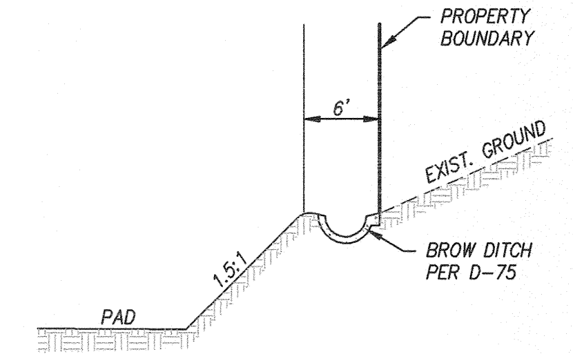
SECTION 'M-M' NOT TO SCALE
