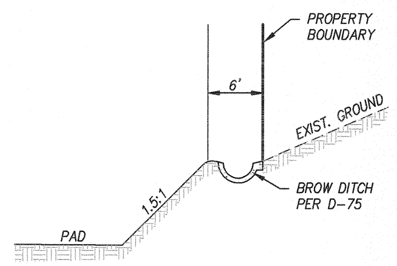
SECTION "M-M" NOT TO SCALE
