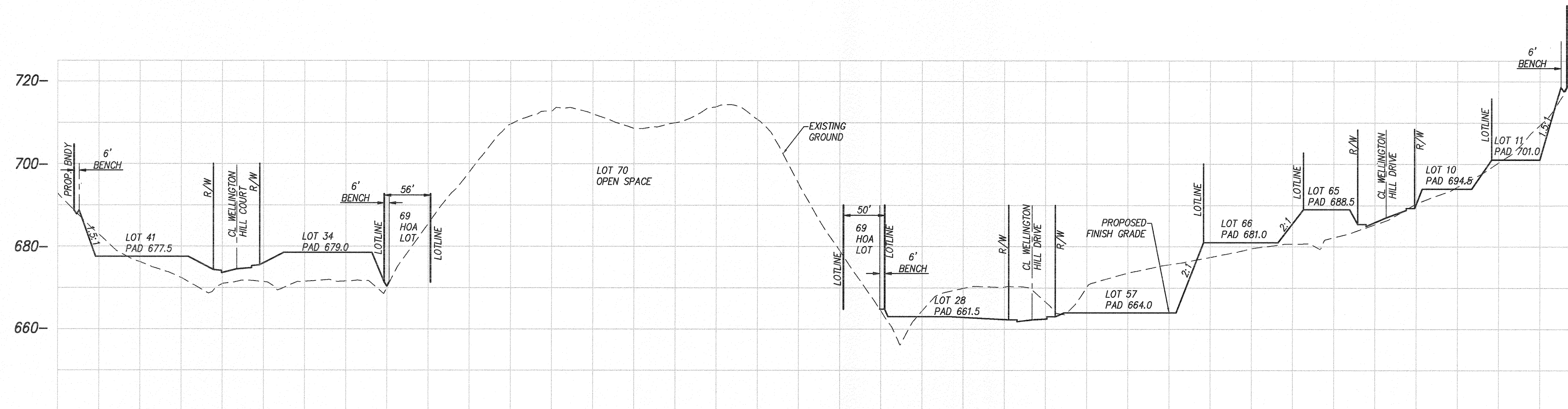
SECTION 'A-A' SCALE H: 1" = 80'; V: 1" = 8'
