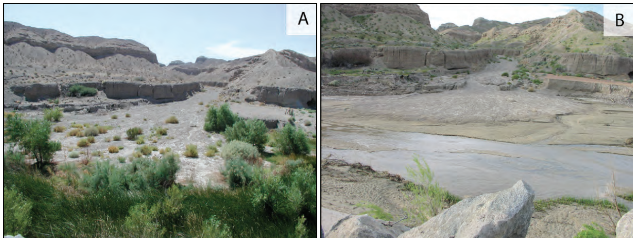
Figure 11. Pre-effective discharge (A) and post-effective discharge (B) on the Mojave River at Afton Canyon. The effective discharge reworked sediment and removed vegetation.
