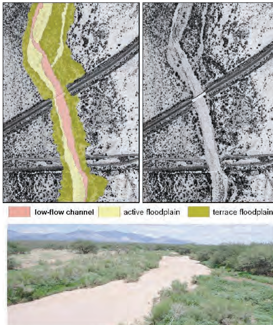
Figure 42. Example geomorphic mapping in a straight reach of a single-thread channel with an adjacent floodplain, Alter Wash, AZ.
