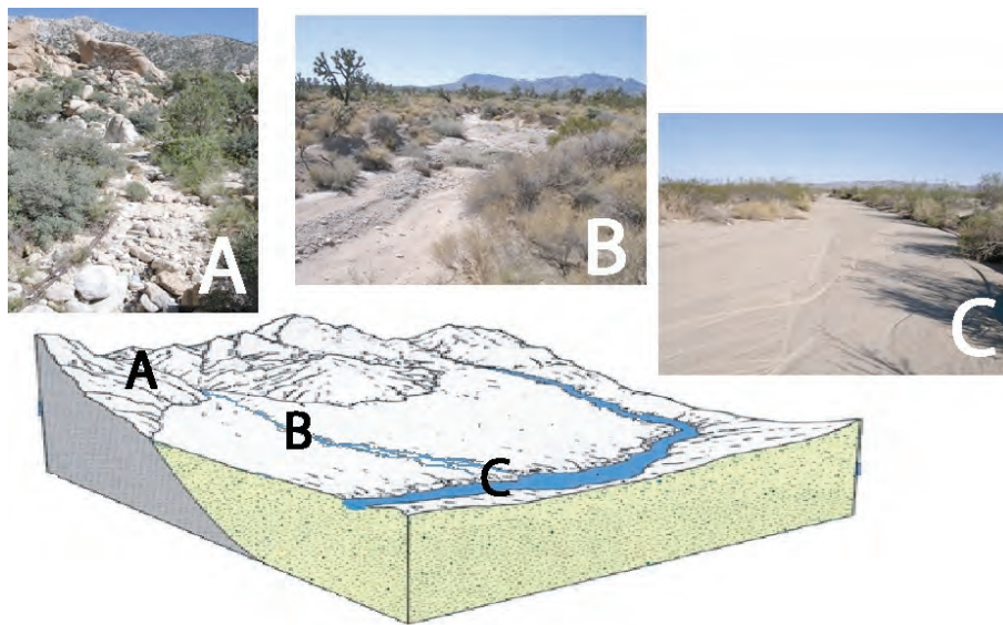
Figure 9. Changes in channel form along an ephemeral stream channel (Caruthers Creek, CA).
