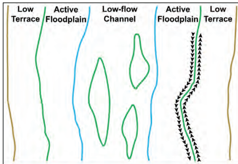
Figure 35. Step 6 of the field verification procedure. The arrows indicate foot paths that should be followed to verify that the transition from the active floodplain to the low terrace identified through observing changes in vegetation, sediment texture, and possibly a break in slope is reliable in both the upstream and downstream directions.
