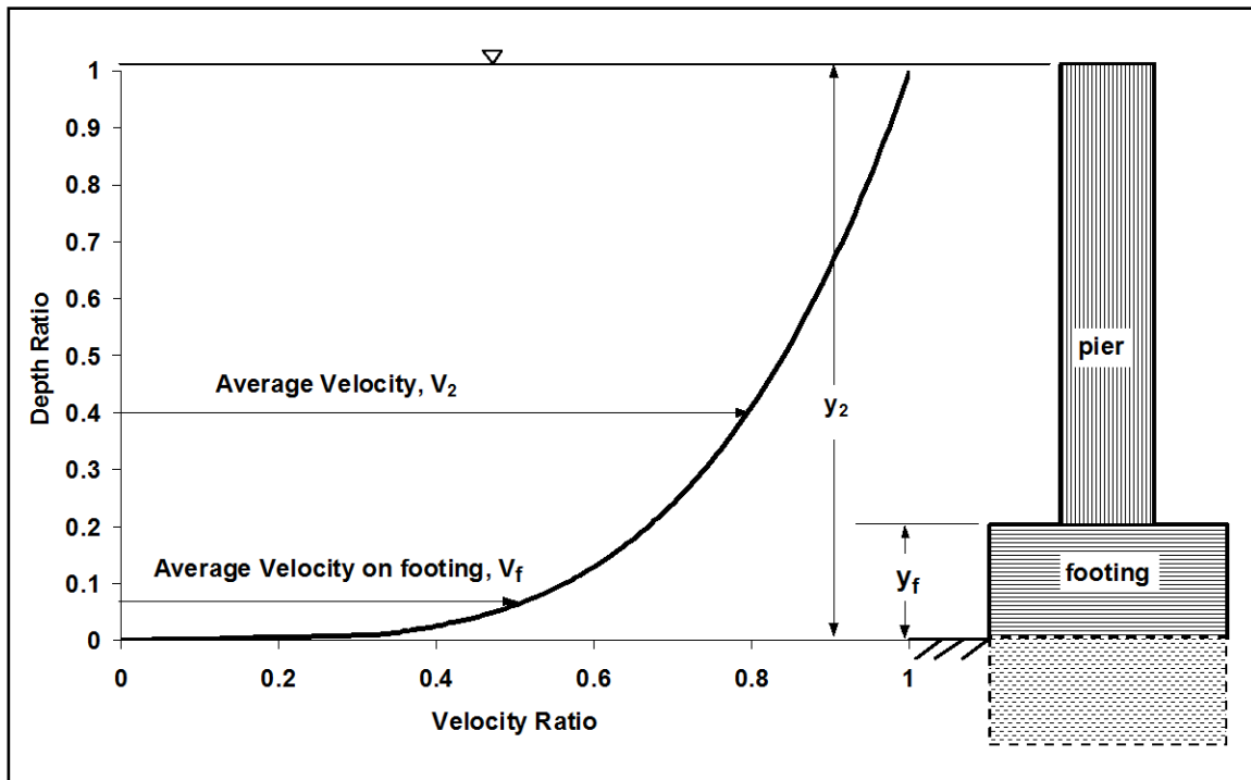
Figure 7.8. Definition sketch for velocity and depth on exposed footing.
