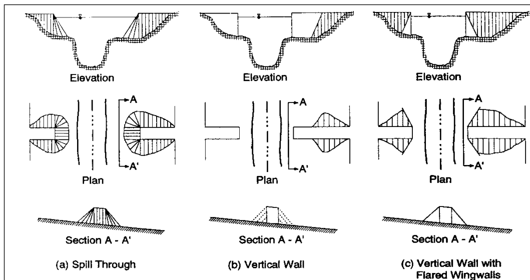
Figure 8.6. Abutment shape.
