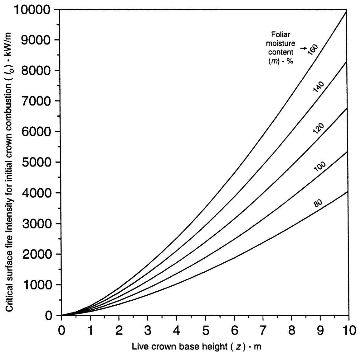
Figure 2.5: Critical surface fire intensity for initial crown combustion in coniferous forest stands as a function of live crown base height and foliar moisture content according to Van Wagner (1977a).
