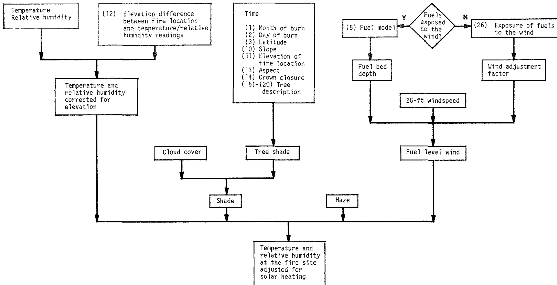
Figure 9.—Flow diagram of the part of the fine fuel moisture model that adjusts temperature and relative humidity for elevation and solar heating. This adjustment is used several places in the model. SITE input values and line numbers are shown at each step.
