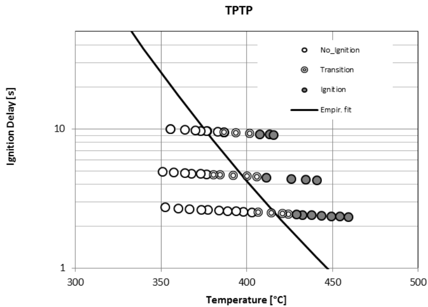
Figure 26. Measured ignition delays for fuel-rich mixtures of TPTP and air. The curve shown is an approximate Arrhenius fit of measured ignition delay time vs. temperature.
