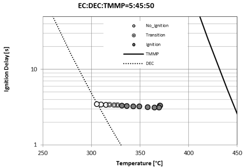
Figure 28. Measured ignition delays for fuel-rich mixtures of 5:45:50 solutions of EC, DEC and TMMP in air.
