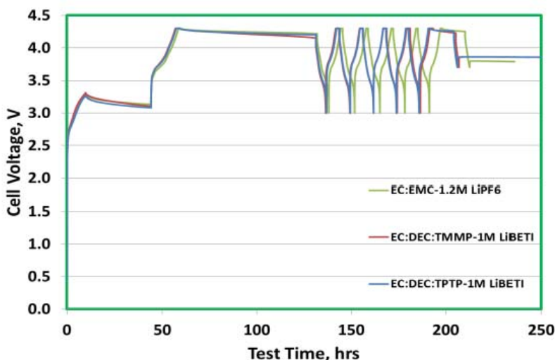
Figure 4. Comparison of 18650 formation cycles for different electrolytes.
