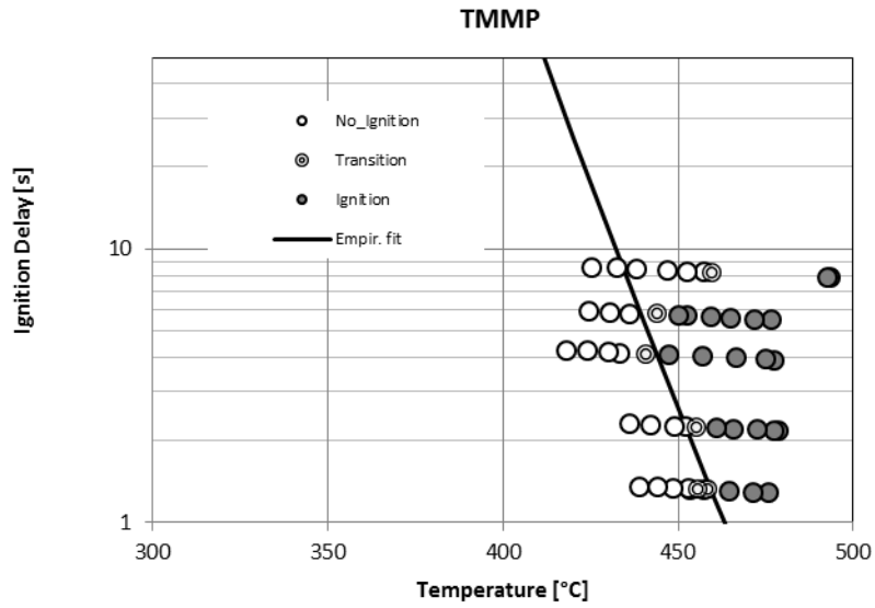
Figure 25. Measured ignition delays for fuel-rich mixtures of TMMP and air. The curve shown is an approximate Arrhenius fit of measured ignition delay time vs. temperature.
