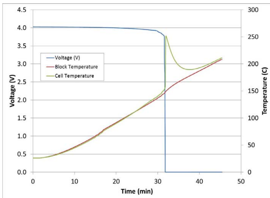
Figure 16. Voltage and temperature data for the TPTP cell during the thermal ramp test.
