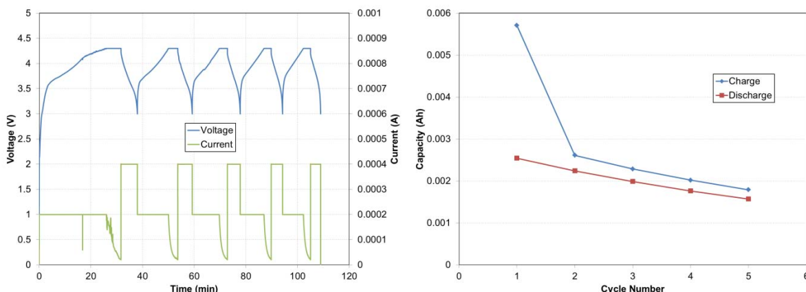
Figure 42. Tabular T64 direct coated separator formation cycling.
