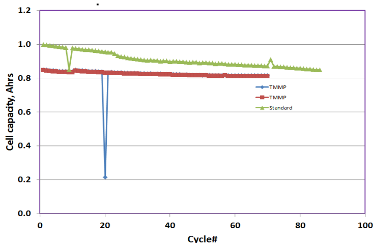
Figure 5. Capacity vs. cycle # for SNL-built 18650 cells containing different electrolytes.
