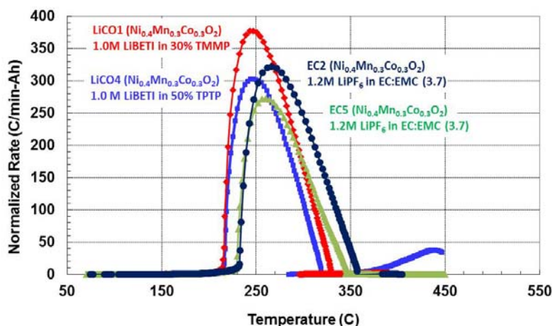
Figure 8. ARC profile for NMC 433/graphite cells with HFE and carbonate electrolytes.
