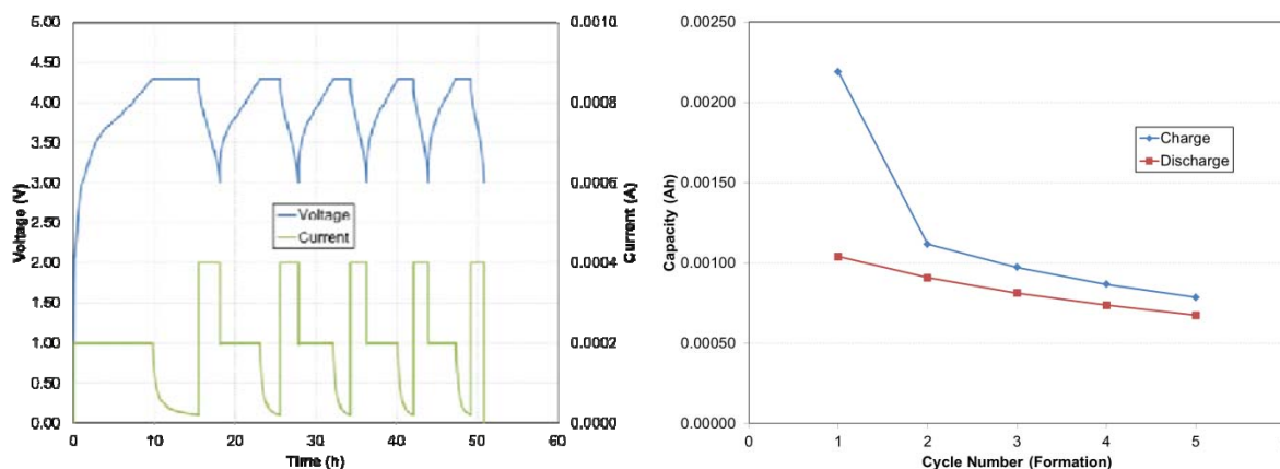
Figure 41. Formation cycling for A3500 SG alumina separator.
