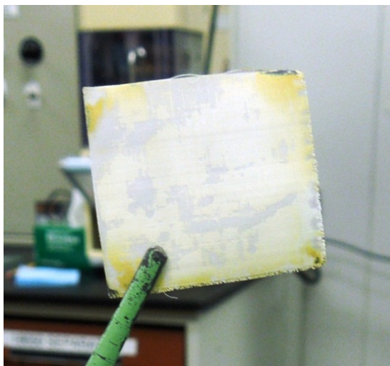
Figure 48. Parylene coated bronze mesh with the mesh dissolved, resulting in a parylene only separator.
