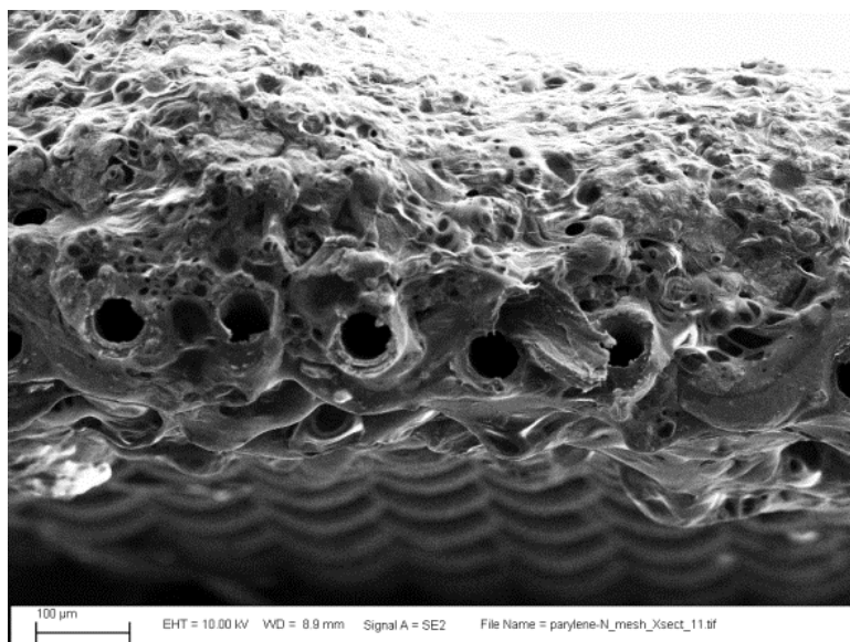
Figure 50. Parylene coated bronze scaffold subsequently etched away, leaving only parylene, then assembled into a coin cell and tested. The holes from the scaffold are visible in the center of the image. The cathode material is visible on the top of the image, and a small section of cathode is visible having extruded onto the anode side of the separator in the bottom right.
