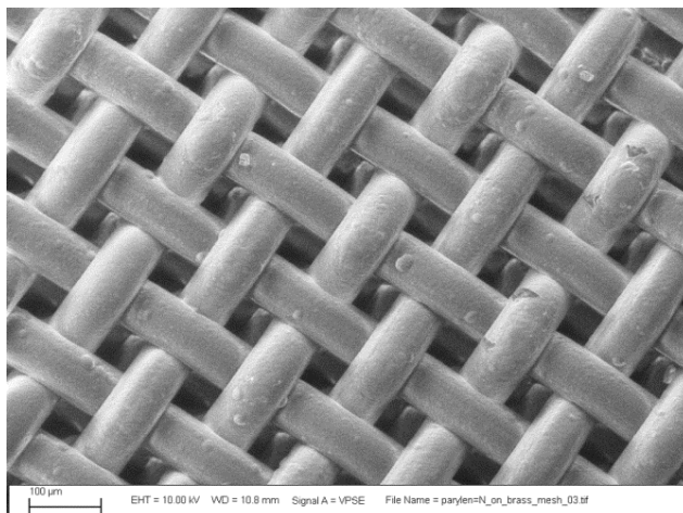
Figure 46. Bronze mesh (50 \mu\text{m} thick wire) after coating with 100 \mu\text{m} of parylene.
