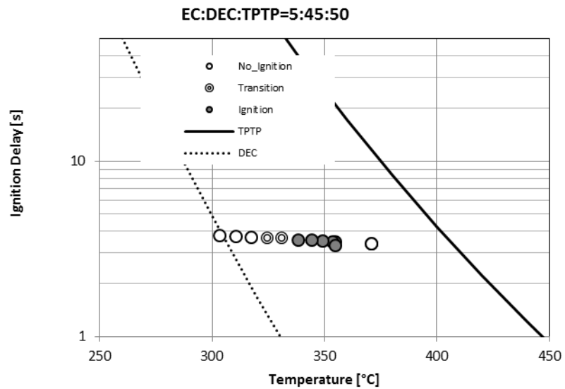
Figure 29. Measured ignition delays for fuel-rich mixtures of 5:45:50 solutions of EC, DEC and TPTP in air.
