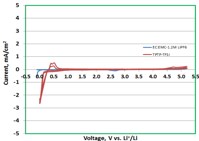
Figure 3. Electrochemical voltage stability window for electrolytes measured at a scan rate of 1 mV/s in a three electrode cell with a platinum working electrode.
