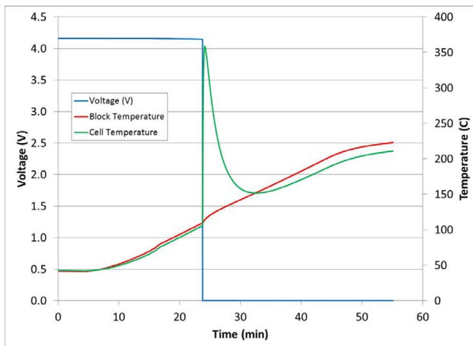
Figure 18. Voltage and temperature data for the TMMP cell during the thermal ramp test.
