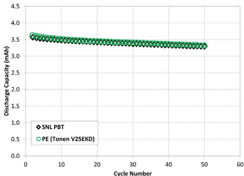
Figure 35. Full cell discharge capacity at C/15 of NMC/Graphite cells in 1.2 M LiPF 6 in EC:EMC (3:7) with SNL PBT separator (black symbol) and commercial PE separator (Tonen) (green symbol).
