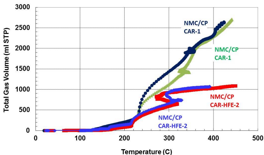
Figure 9. HFE electrolytes in 18650 NMC 433/graphite cells show lower gas volume than the baseline.
