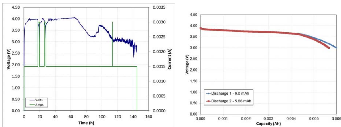
Figure 51. Formation cycle of with parylene coated bronze scaffold, with the scaffold etched away (left) and discharge capacity of the cell during the first two successful cycles (right).
