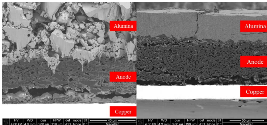
Figure 43. SEM cross-sections of T64 tabular alumina (left) and AKP53 alumina (right) separator coated directly onto the anode.
