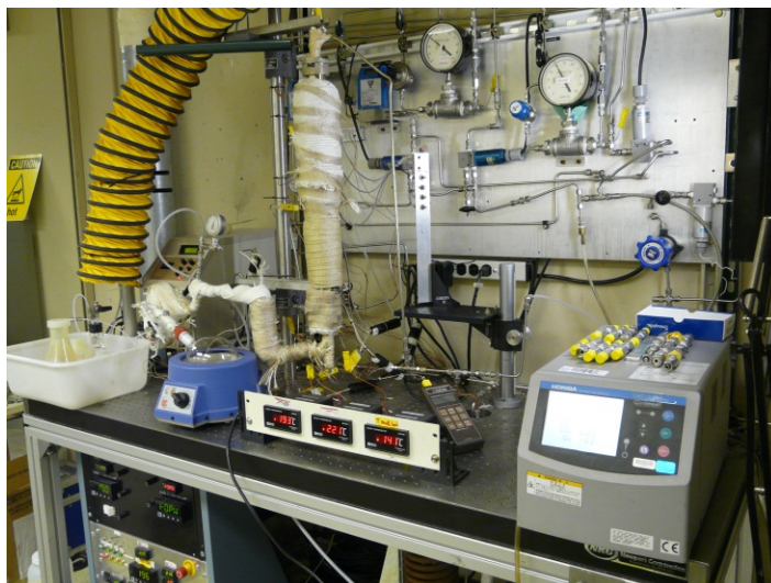
Figure 20. Photograph of the experimental setup, with liquid supply and HPLC pump to the left, insulated reactor tube in the middle, and gas analyzer to the right.
