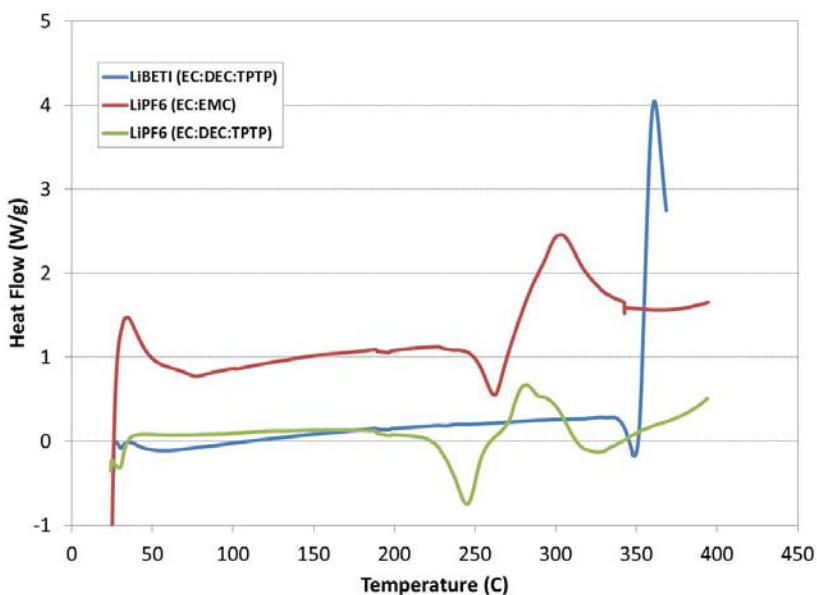
Figure 6. DSC measurements of heat flow (W/g) as a function of temperature for HFE/sulfonimide and carbonate/LiPF 6 electrolytes.
