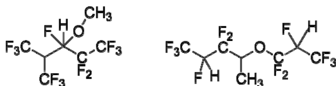
Figure 1. Chemical structures for 2-trifluoromethyl-3-methoxyperfluoropentane (TMMP) (left) and 2-trifluoro-2-fluoro-3-difluoropropoxy-3-difluoro-4-fluoro-5-trifluoropentane (TTPP) (right) hydrofluoro ethers used for evaluation.
