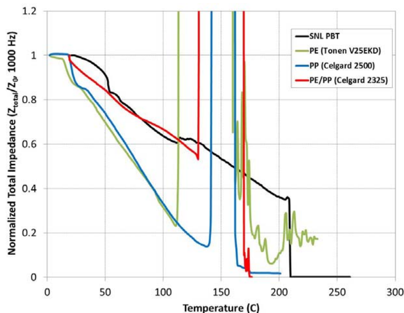
Figure 38. Normalized separator AC impedance ( Z_{\text{total}}/Z_0 , 1000 Hz) as a function of temperature for SNL PBT separator (black trace), PE separator (green trace), PP (blue trace), and multilayer PE/PP separator (red trace).
