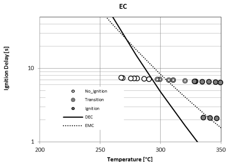
Figure 24. Measured ignition delays for fuel-rich mixtures of ethylene carbonate and air. The curves shown are approximate Arrhenius fit of measured ignition delay time vs. temperature for DEC and EMC.
