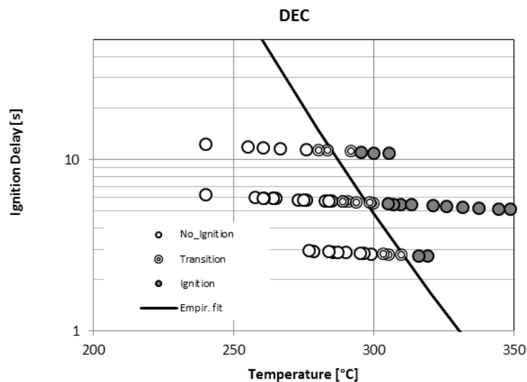
Figure 22. Measured ignition delays for fuel-rich mixtures of diethyl carbonate and air. The curve shown is an approximate Arrhenius fit of measured ignition delay time vs. temperature.
