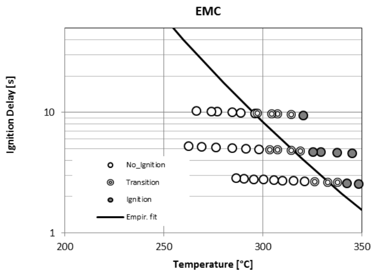
Figure 23. Measured ignition delays for fuel-rich mixtures of ethyl methyl carbonate and air. The curve shown is an approximate Arrhenius fit of measured ignition delay time vs. temperature.
