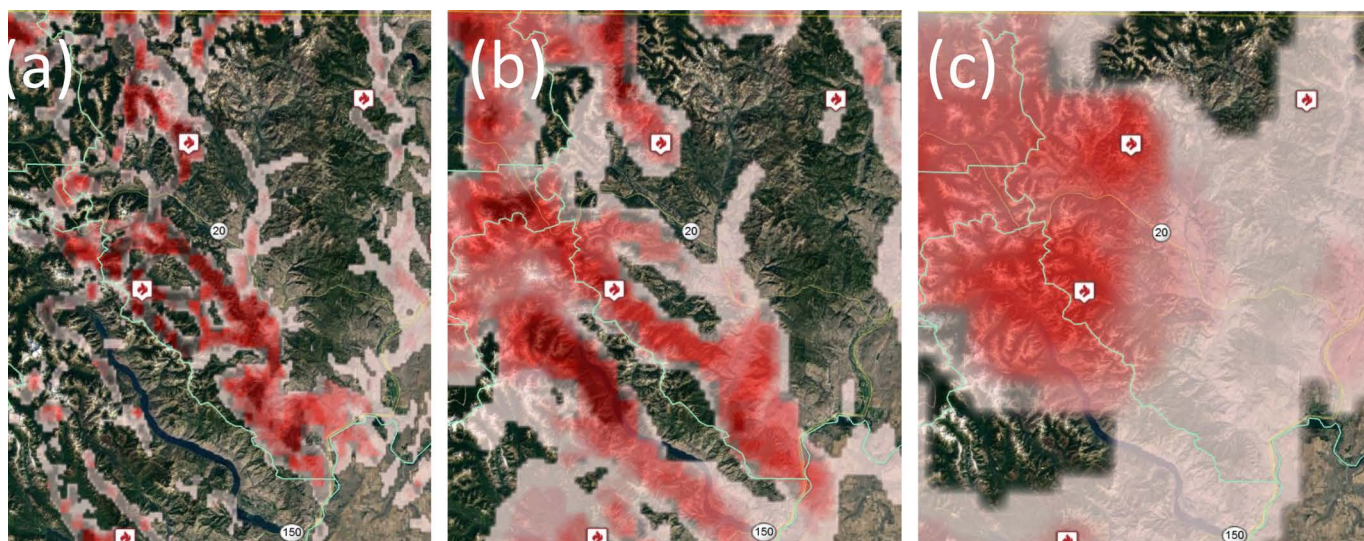
Figure C6. BlueSky hourly average surface smoke predictions at 1 am on 8/19/2018 at 3 grid resolutions: (a) 1.33 km, (b) 4 km, and (c) 12 km in north central Washington. Higher resolution versions (a and b) allow the effect of complex terrain to be better reflected in smoke concentration estimates. KML/Google Earth version.
