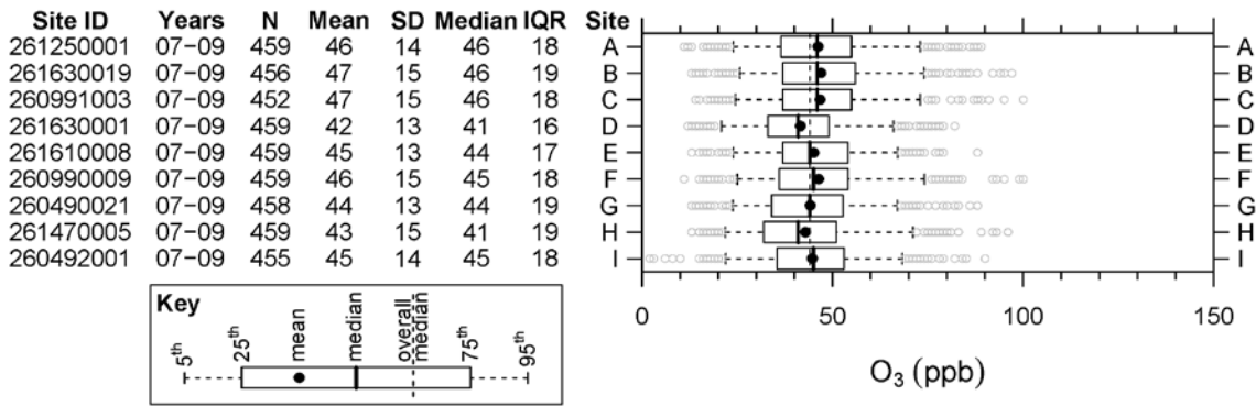
Figure 3-103 Site information, statistics and box plots for 8-h daily max O 3 from AQS monitors meeting the warm-season data set inclusion criteria within the Detroit, Michigan, CSA.
