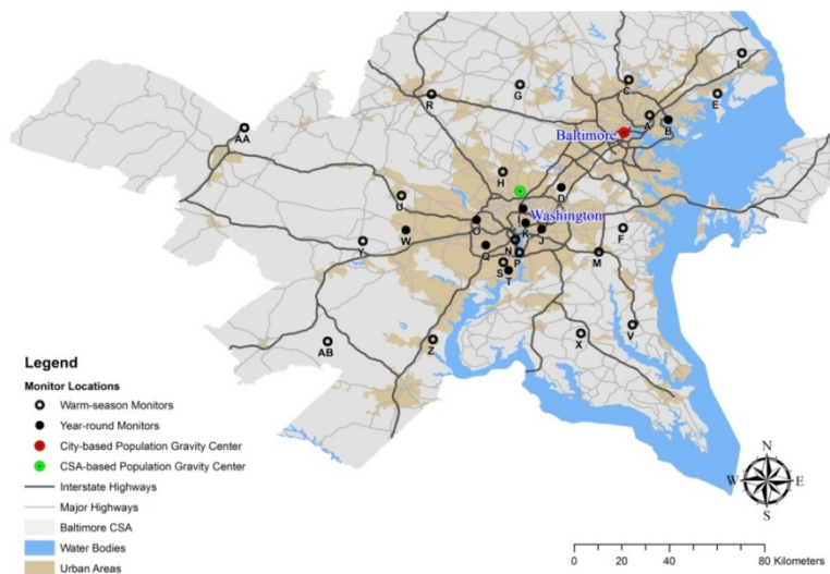
Figure 3-77 Map of the Baltimore, Maryland, CSA including O 3 monitor locations, population gravity centers, urban areas, and major roadways.
