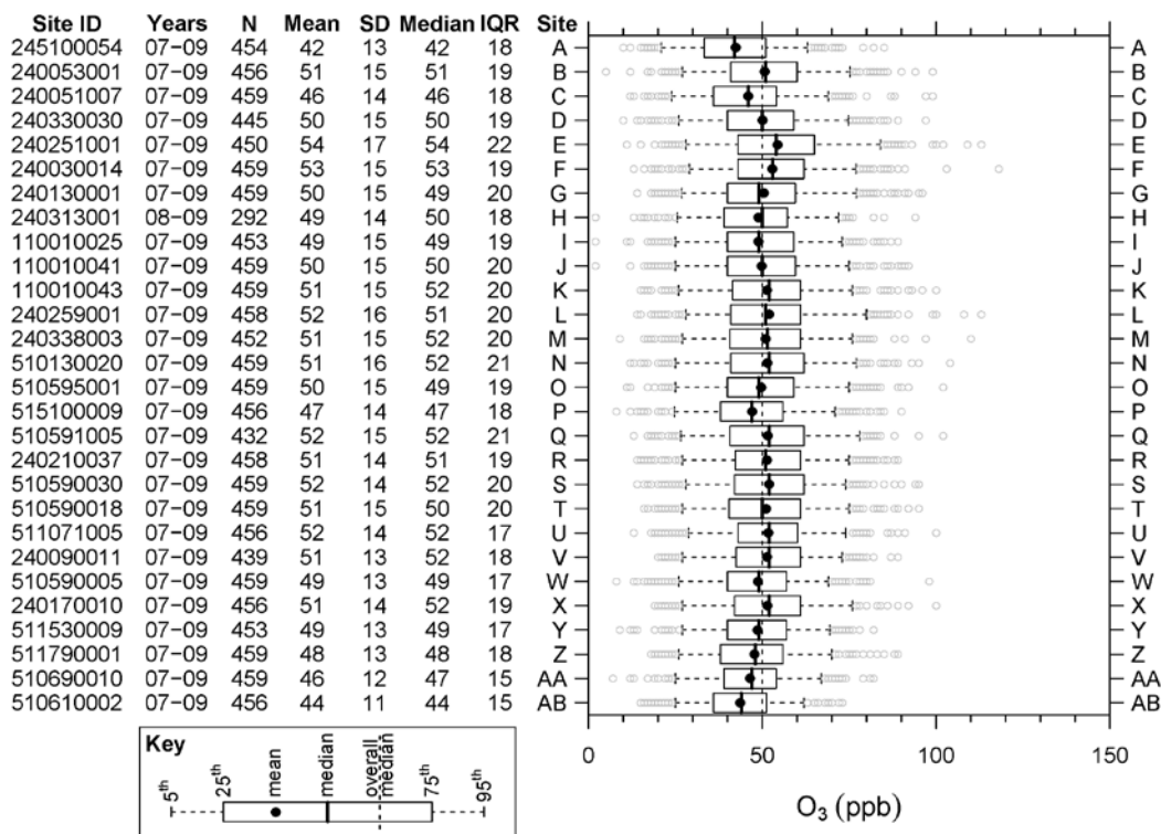
Figure 3-97 Site information, statistics and box plots for 8-h daily max O 3 from AQS monitors meeting the warm-season data set inclusion criteria within the Baltimore, Maryland, CSA.
