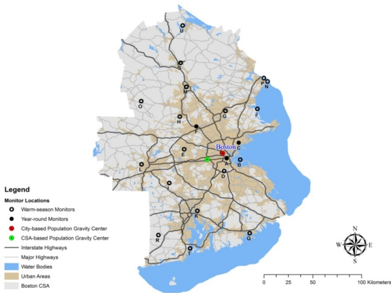
Figure 3-79 Map of the Boston, Massachusetts, CSA including O 3 monitor locations, population gravity centers, urban areas, and major roadways.
