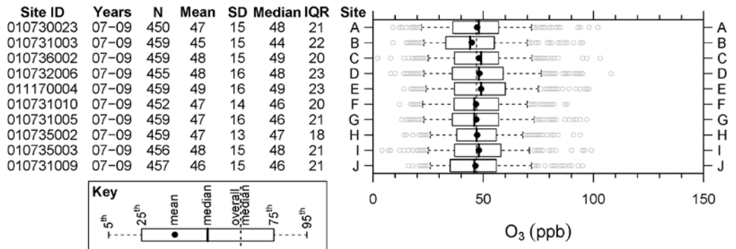
Figure 3-98 Site information, statistics and box plots for 8-h daily max O 3 from AQS monitors meeting the warm-season data set inclusion criteria within the Birmingham, Alabama, CSA.
