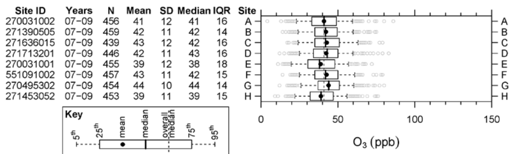
Figure 3-106 Site information, statistics and box plots for 8-h daily max O 3 from AQS monitors meeting the warm-season data set inclusion criteria within the Minneapolis, Minnesota, CSA.
