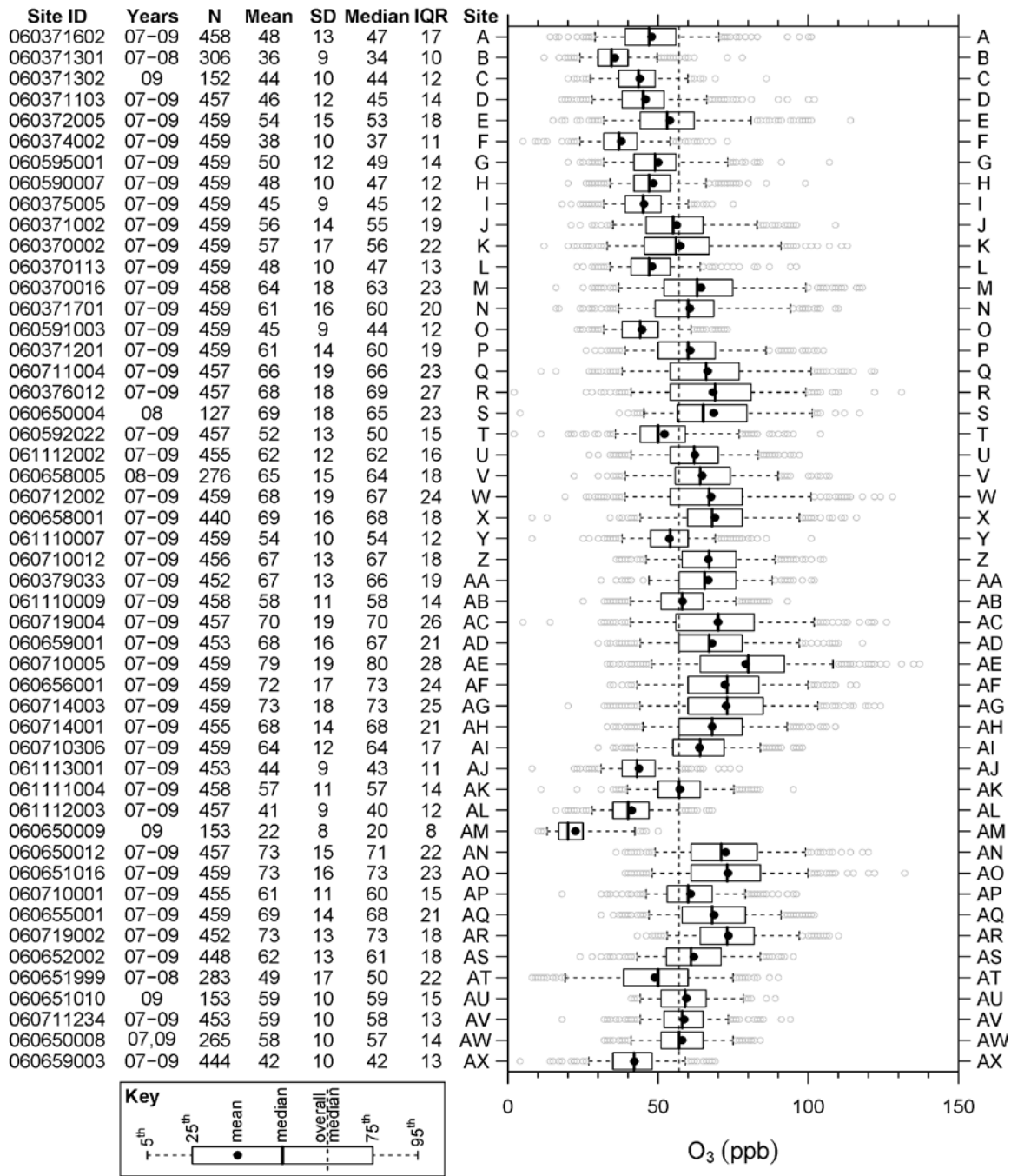
Figure 3-34 Site information, statistics and box plots for 8-h daily max O 3 from AQS monitors meeting the warm-season data set inclusion criteria within the Los Angeles CSA.
