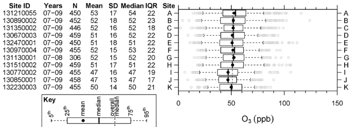
Figure 3-32 Site information, statistics and box plots for 8-h daily max O 3 from AQS monitors meeting the warm-season data set inclusion criteria within the Atlanta CSA.
