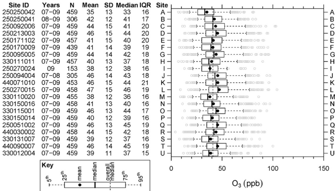
Figure 3-33 Site information, statistics and box plots for 8-h daily max O 3 from AQS monitors meeting the warm-season data set inclusion criteria within the Boston CSA.
