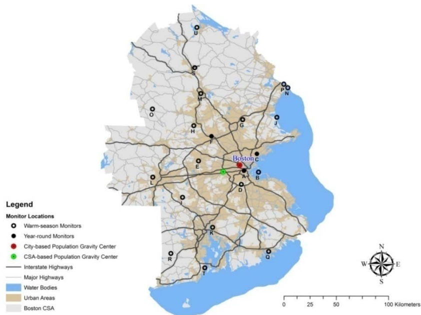
Figure 3-30 Map of the Boston, Massachusetts, CSA including O 3 monitor locations, population gravity centers, urban areas, and major roadways.
