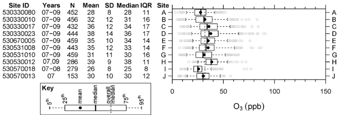
Figure 3-114 Site information, statistics and box plots for 8-h daily max O 3 from AQS monitors meeting the warm-season data set inclusion criteria within the Seattle, Washington, CSA.
