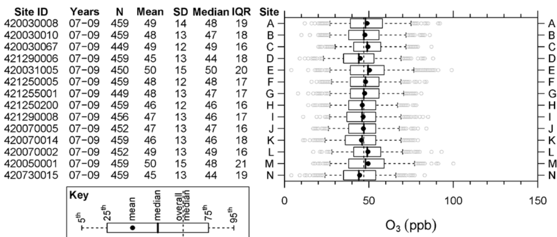
Figure 3-110 Site information, statistics and box plots for 8-h daily max O 3 from AQS monitors meeting the warm-season data set inclusion criteria within the Pittsburgh, Pennsylvania, CSA.
