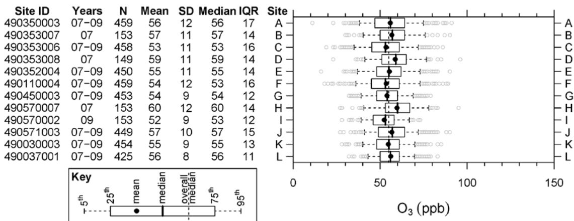
Figure 3-111 Site information, statistics and box plots for 8-h daily max O 3 from AQS monitors meeting the warm-season data set inclusion criteria within the Salt Lake City, Utah, CSA.
