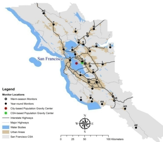
Figure 3-93 Map of the San Francisco, California, CSA including O 3 monitor locations, population gravity centers, urban areas, and major roadways.
