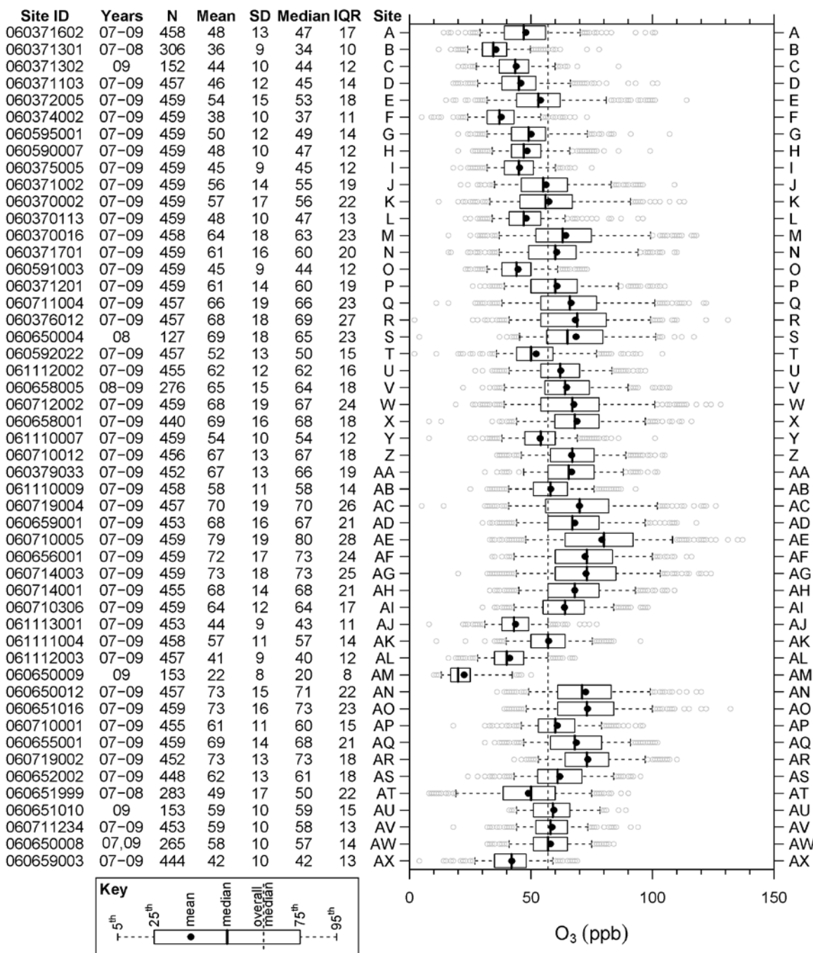
Figure 3-105 Site information, statistics and box plots for 8-h daily max O 3 from AQS monitors meeting the warm-season data set inclusion criteria within the Los Angeles, California, CSA.
