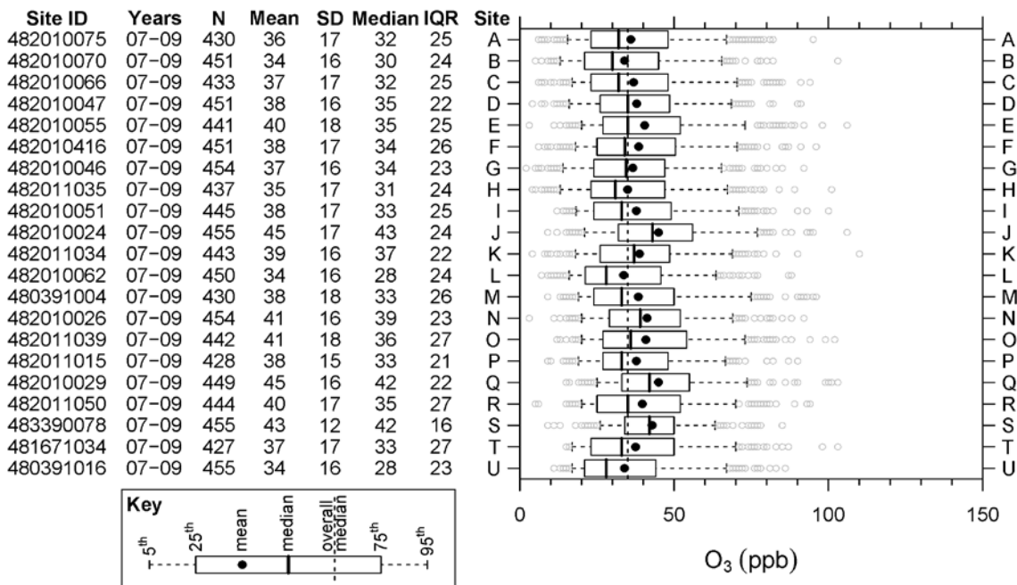
Figure 3-104 Site information, statistics and box plots for 8-h daily max O 3 from AQS monitors meeting the warm-season data set inclusion criteria within the Houston, Texas, CSA.
