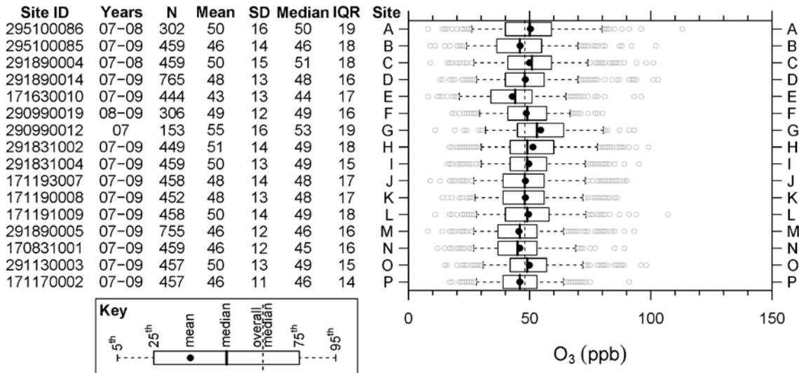
Figure 3-115 Site information, statistics and box plots for 8-h daily max O 3 from AQS monitors meeting the warm-season data set inclusion criteria within the St. Louis, Missouri, CSA.
