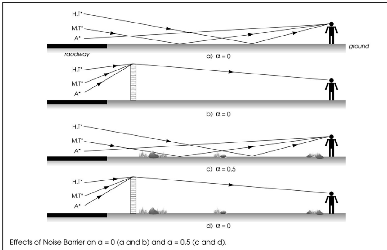
Figure 5-16. Ground Effects
