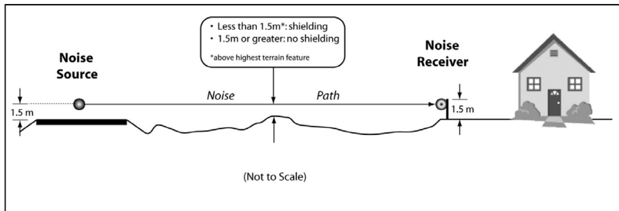
Figure 4-1. Shielding Criterion
