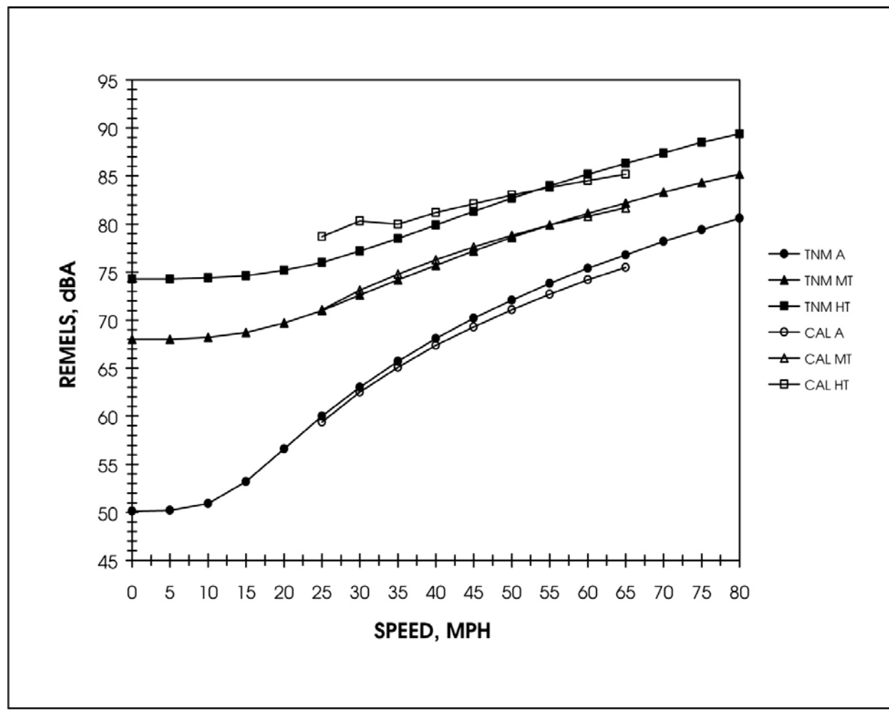
Figure 5-17. Comparison of A-Weighted Baseline FHWA TNM vs. Calveno REMELs
