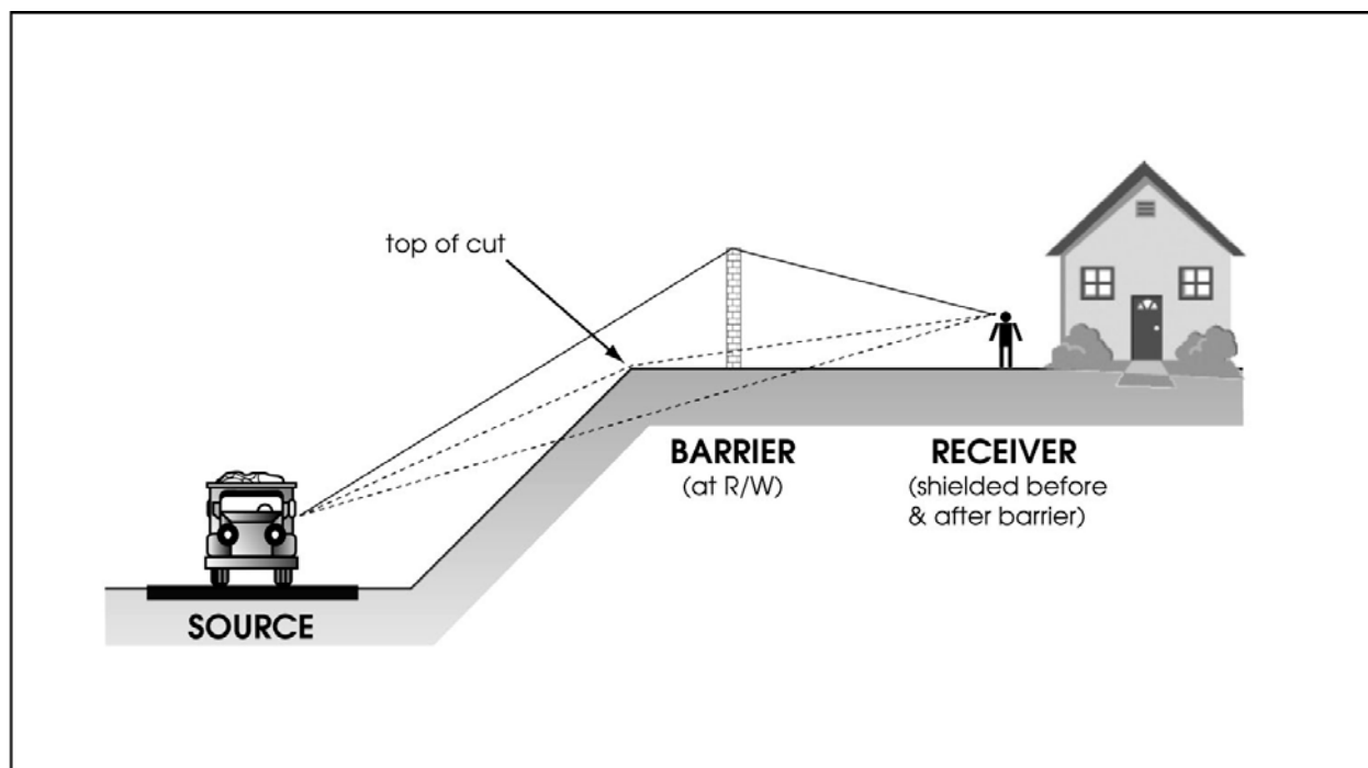
Figure 6-5. Typical Barrier Location for Depressed Highways
