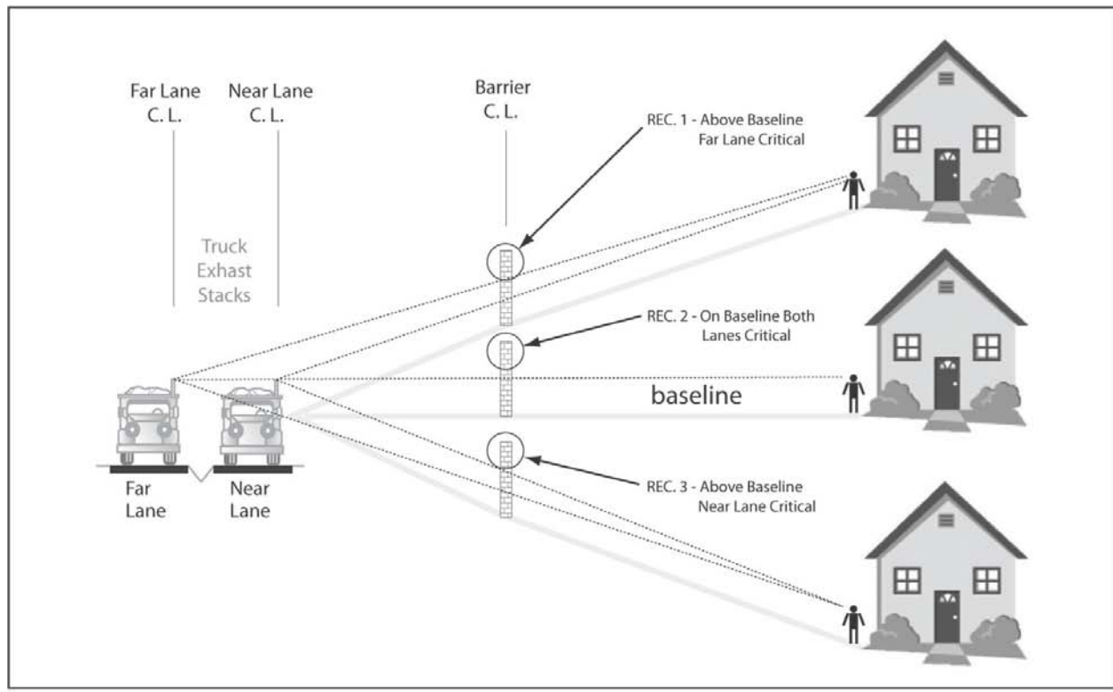
Figure 6-15. Determination of Critical Lane for Line-of-Sight Height (Consult Online Version of Highway Design Manual Chapter 1100 for Latest Status or Changes in Line-of-Sight Guidance)
