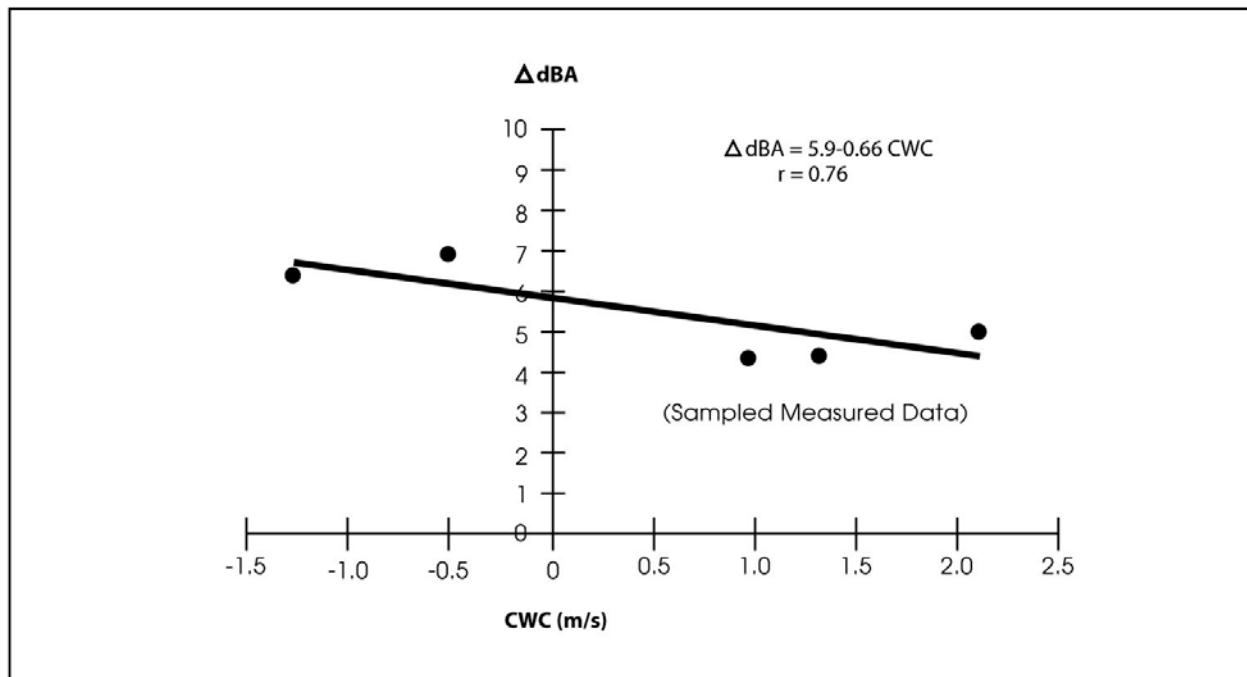
Figure 5-5. \Delta dBA vs. Crosswind Component Linear Regression from Table 5-8 Data
