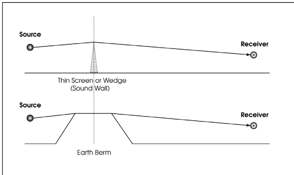
Figure 6-20. Thin Screen vs. Berm (Berm Gives More Barrier Attenuation)
