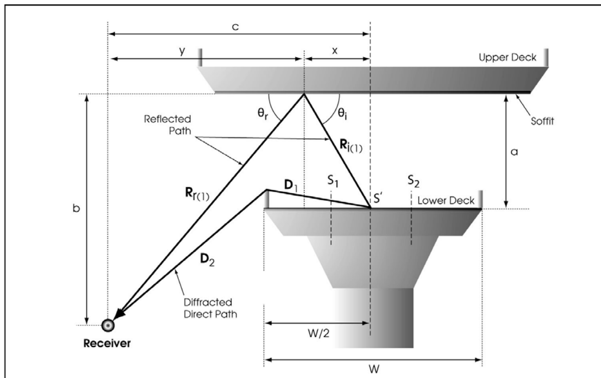
Figure 6-35. Double-Deck Structure Reflections, First Reflective Path
