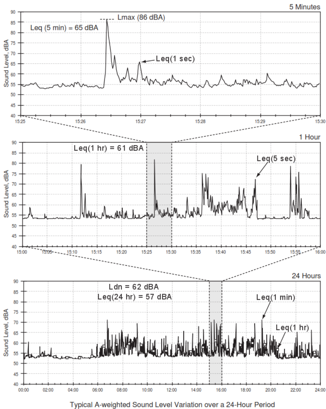
Figure B-10 Example A-weighted Sound Level Time Histories
