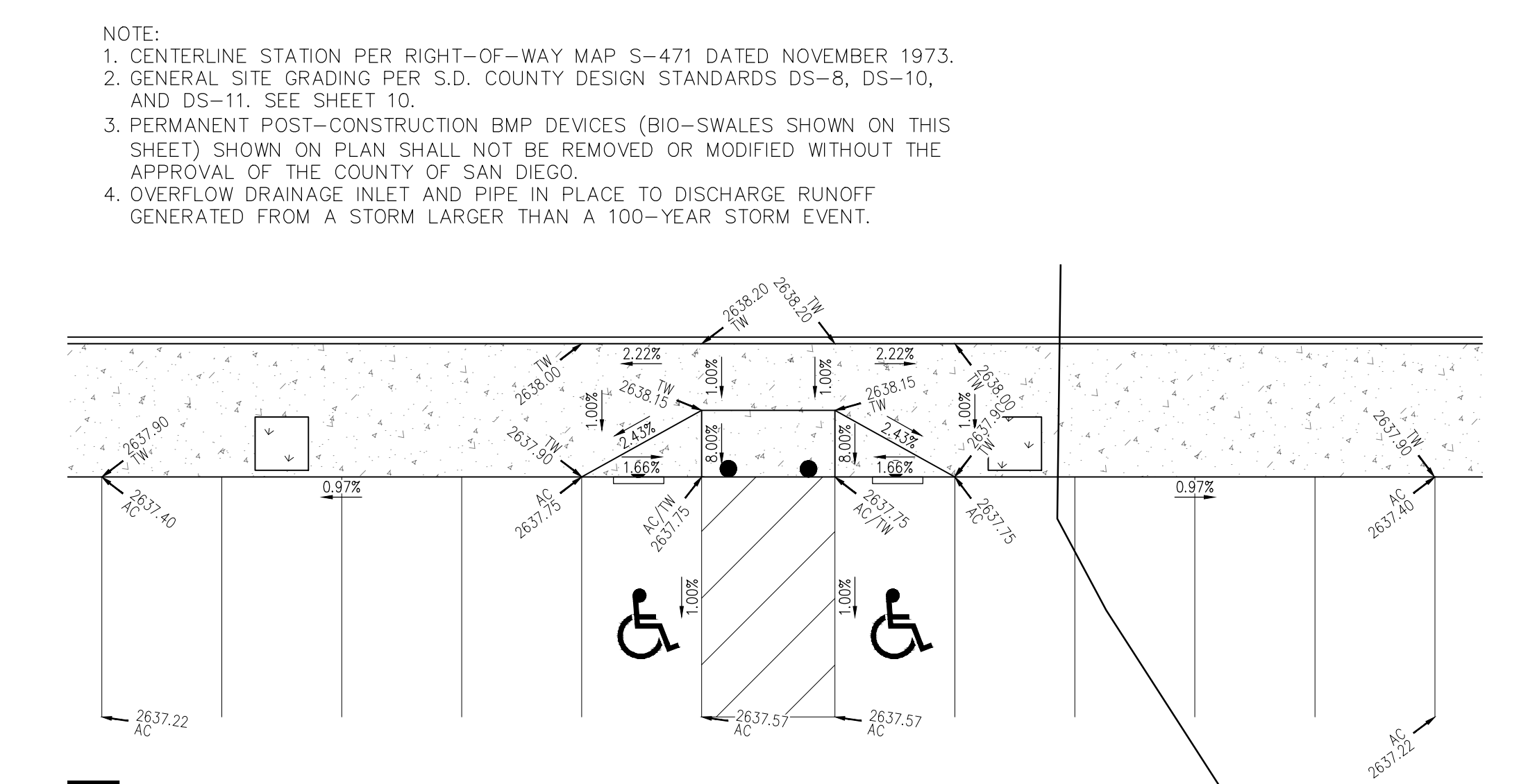
2 ACCESSIBLE RAMP DETAIL 1"=10'
