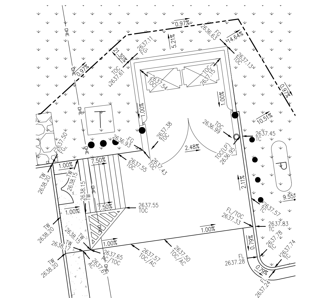
1 TRASH ENCLOSURE & RAMP DETAIL 1"=10'
