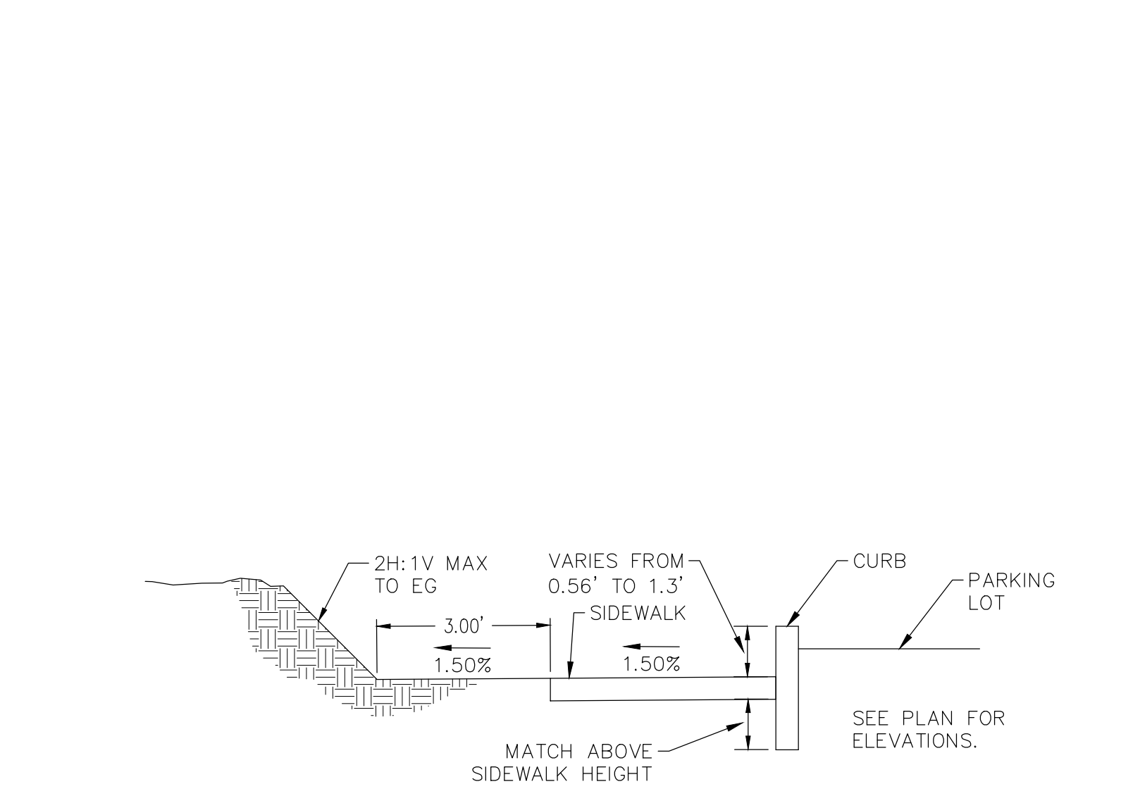
3 SIDEWALK DETAIL NTS
