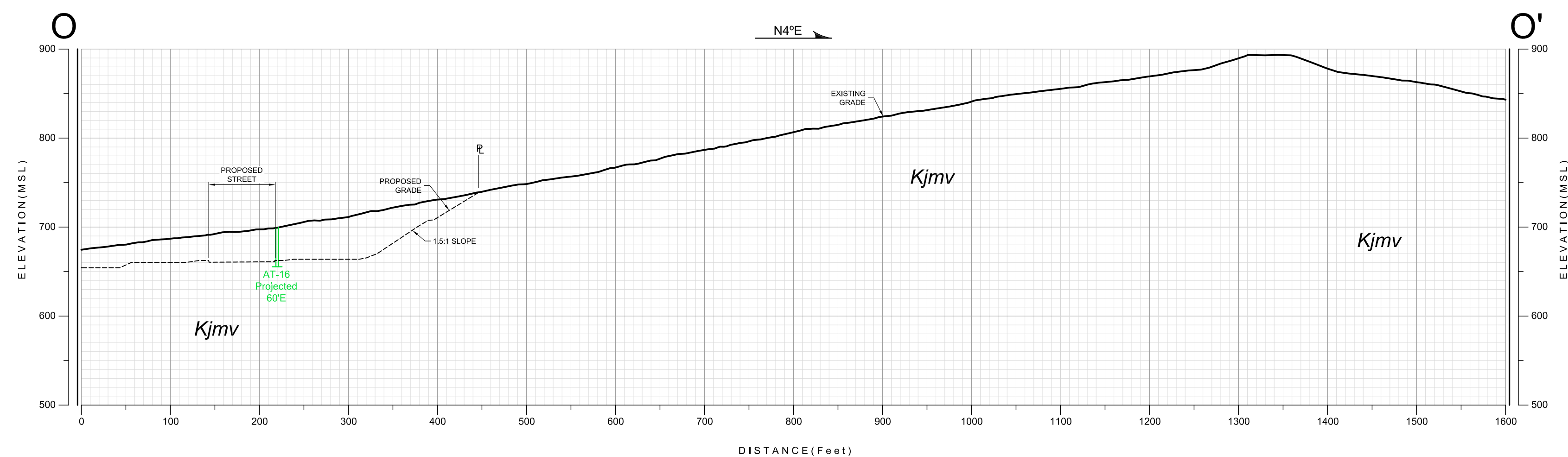
GEOLOGIC CROSS-SECTION O-O' SCALE: 1" = 100' (Vert. = Horiz.)
