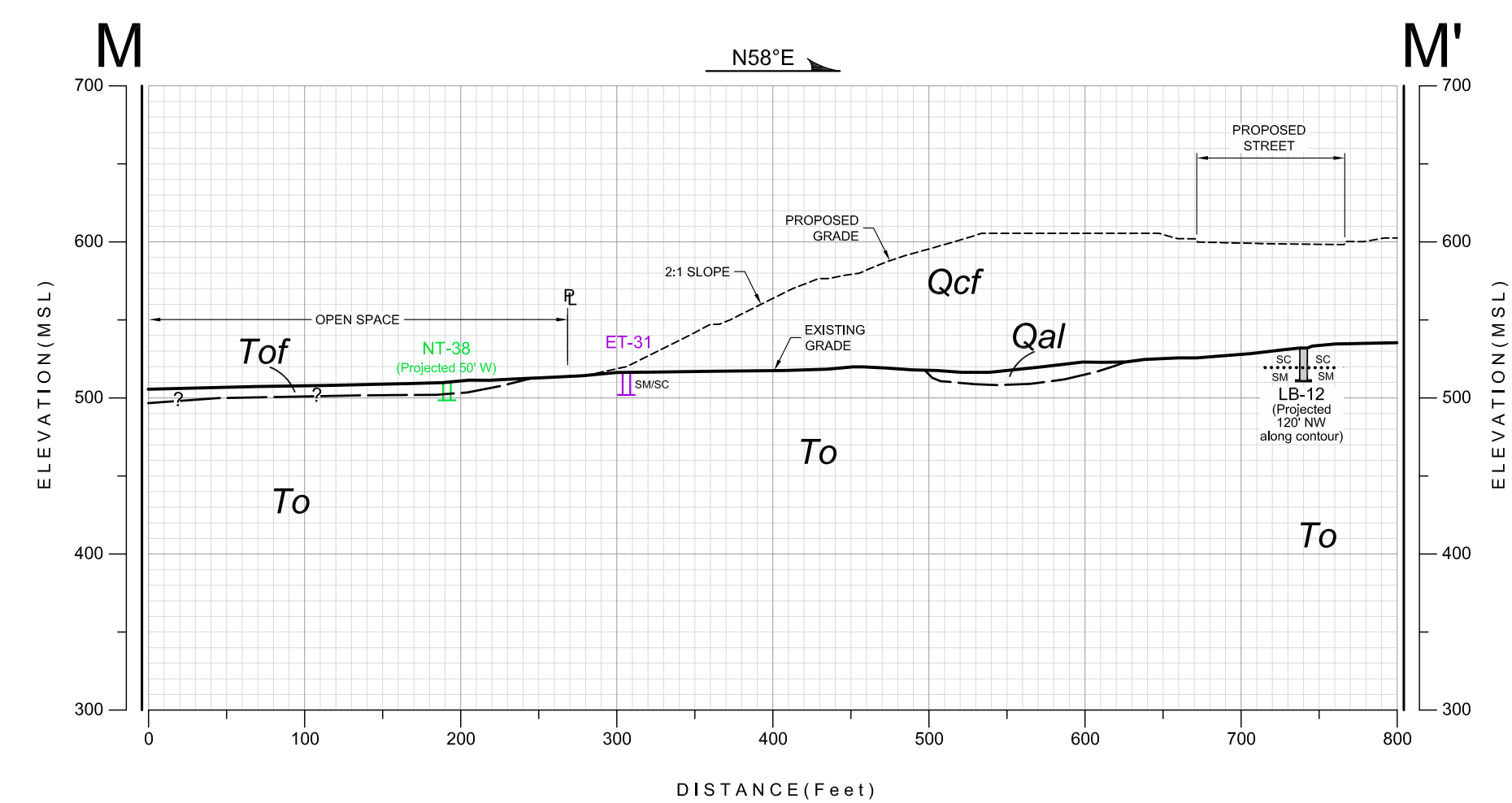
GEOLOGIC CROSS-SECTION M-M' SCALE: 1" = 100' (Vert. = Horiz.)
