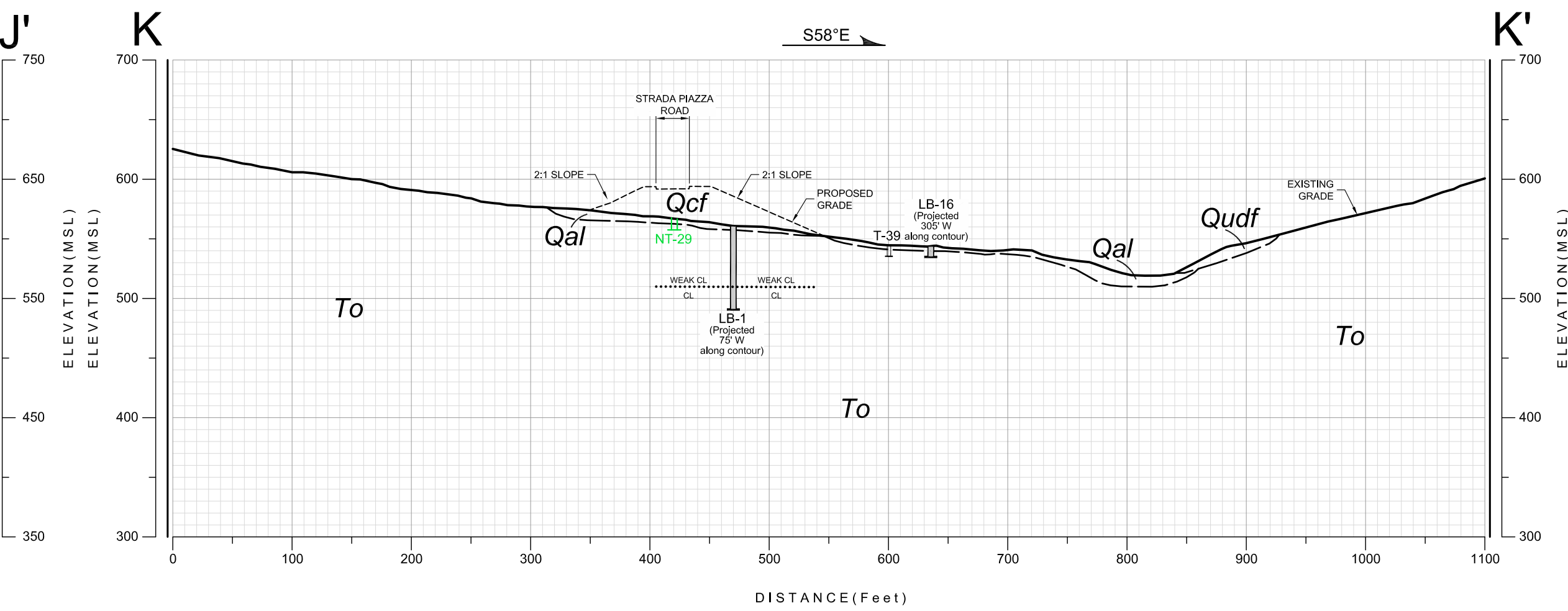
GEOLOGIC CROSS-SECTION K-K' SCALE: 1" = 100' (Vert. = Horiz.)
