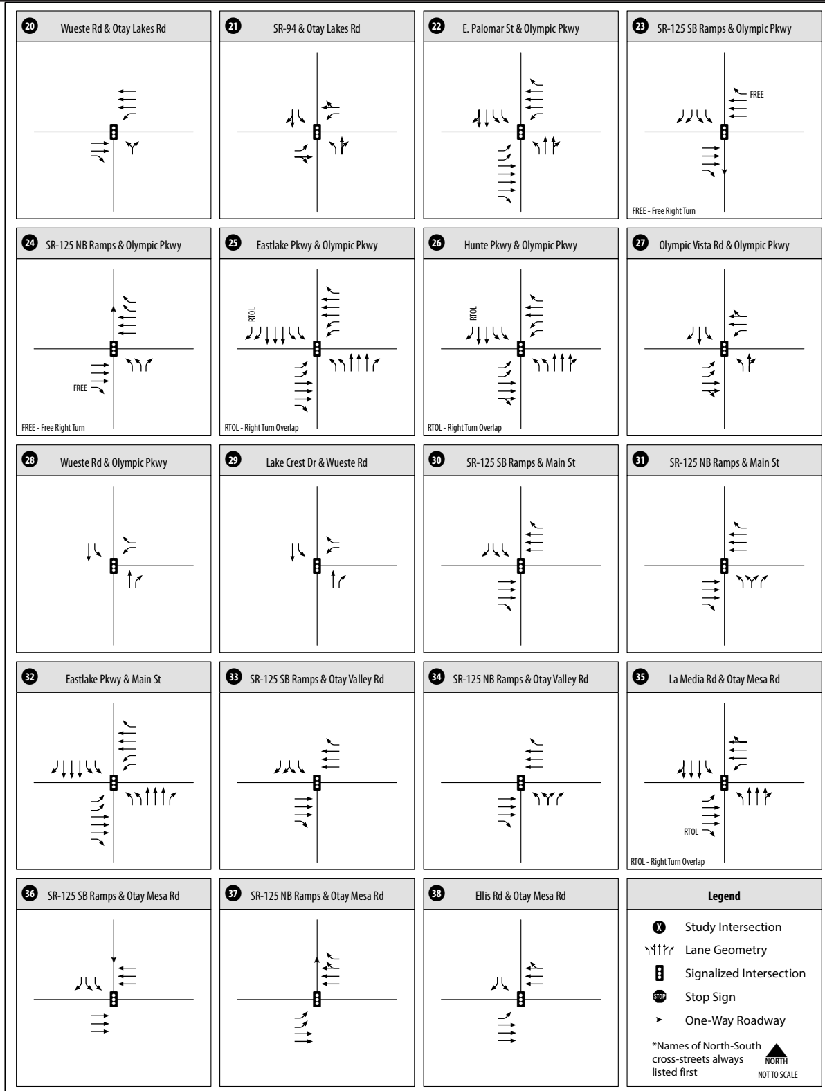
Figure 2.9-25 Intersection Geometrics - Future Year 2030 Conditions (Intersections 20-38)
