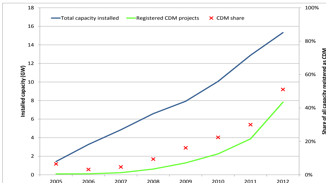
Figure 4-3: Total cumulated wind power capacity installed in India between 2005 and 2012
