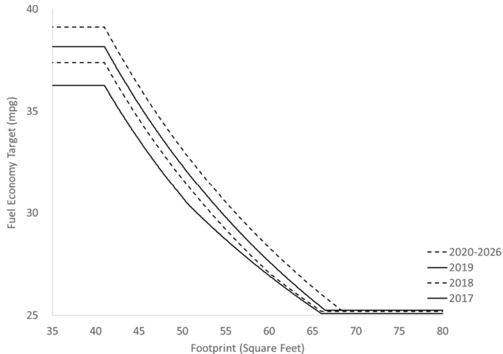
Figure III-3 - Light Truck Fuel Economy Targets
