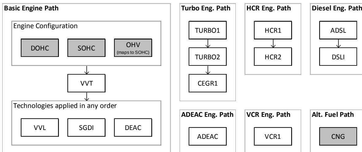
Figure-II-13 - Engine Paths
