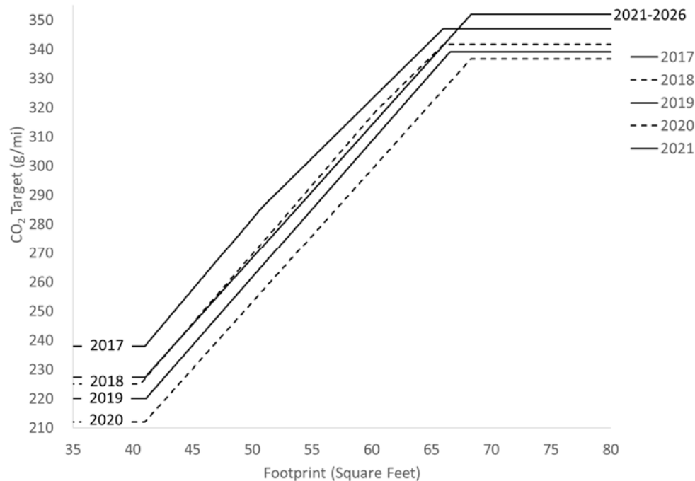
Figure III-4 - Light Truck CO 2 Targets 378
