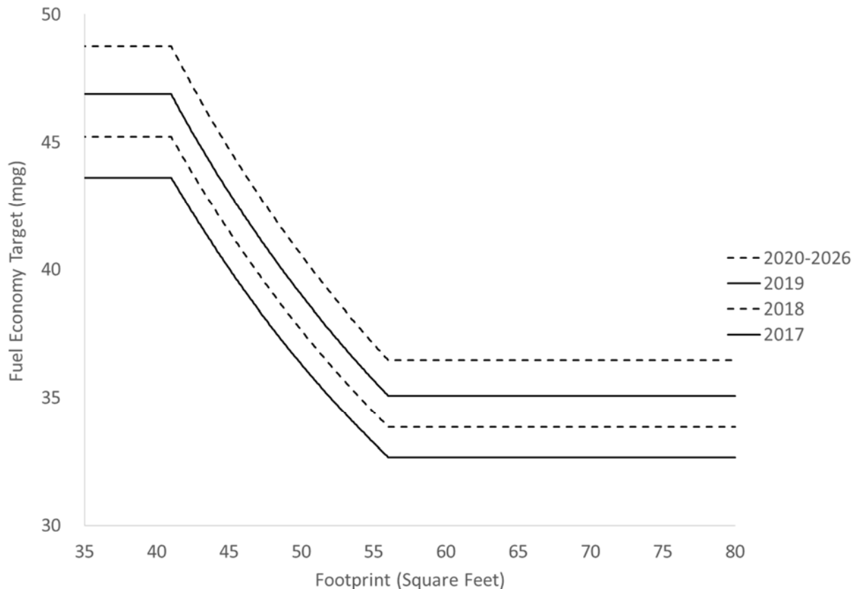
Figure III-1 -Passenger Car Fuel Economy Targets
