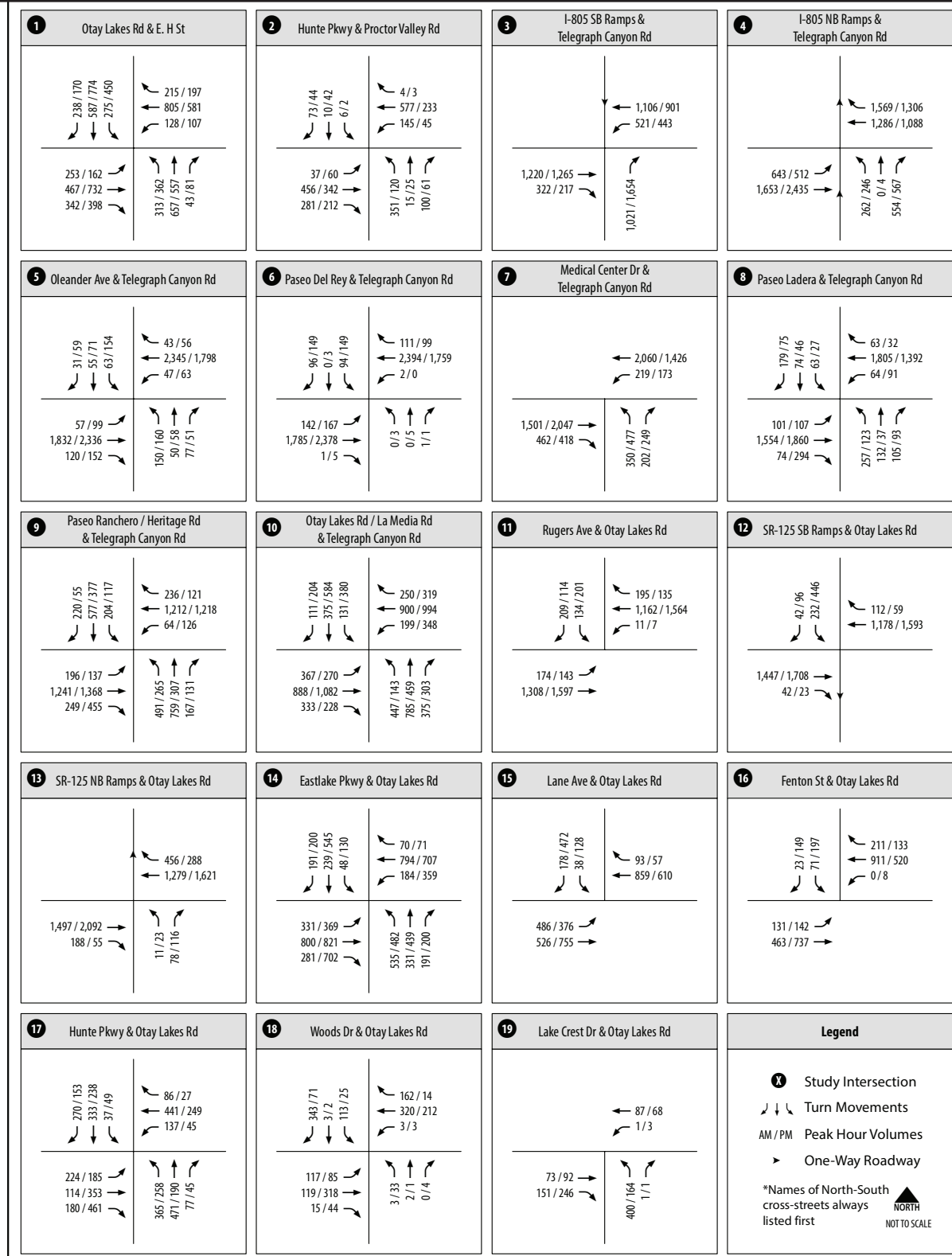
Figure 2.9-15 Intersection Peak Hour Traffic Volumes - Existing Conditions (Intersections 1-19)
