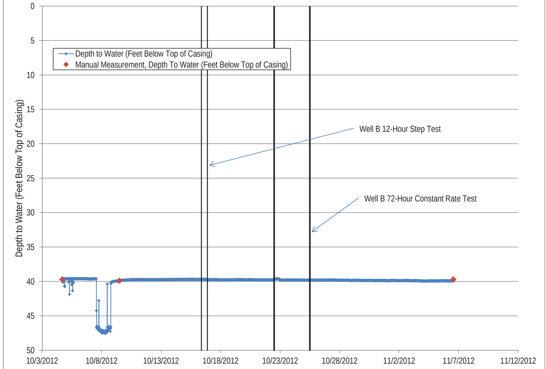
Figure 20. Off-site Well GS-1 Water Level Data
