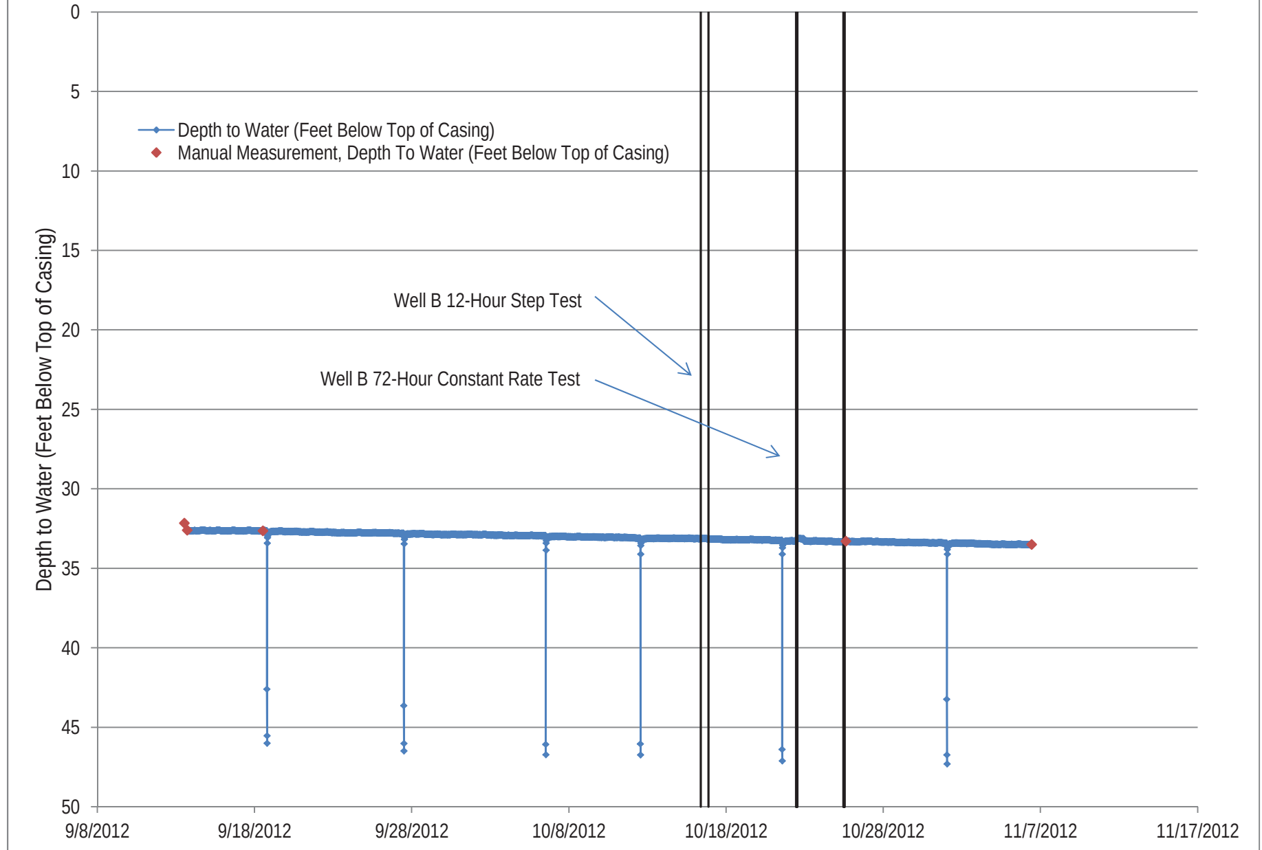
Figure 22. Off-site Well LK-1 Water Level Data
