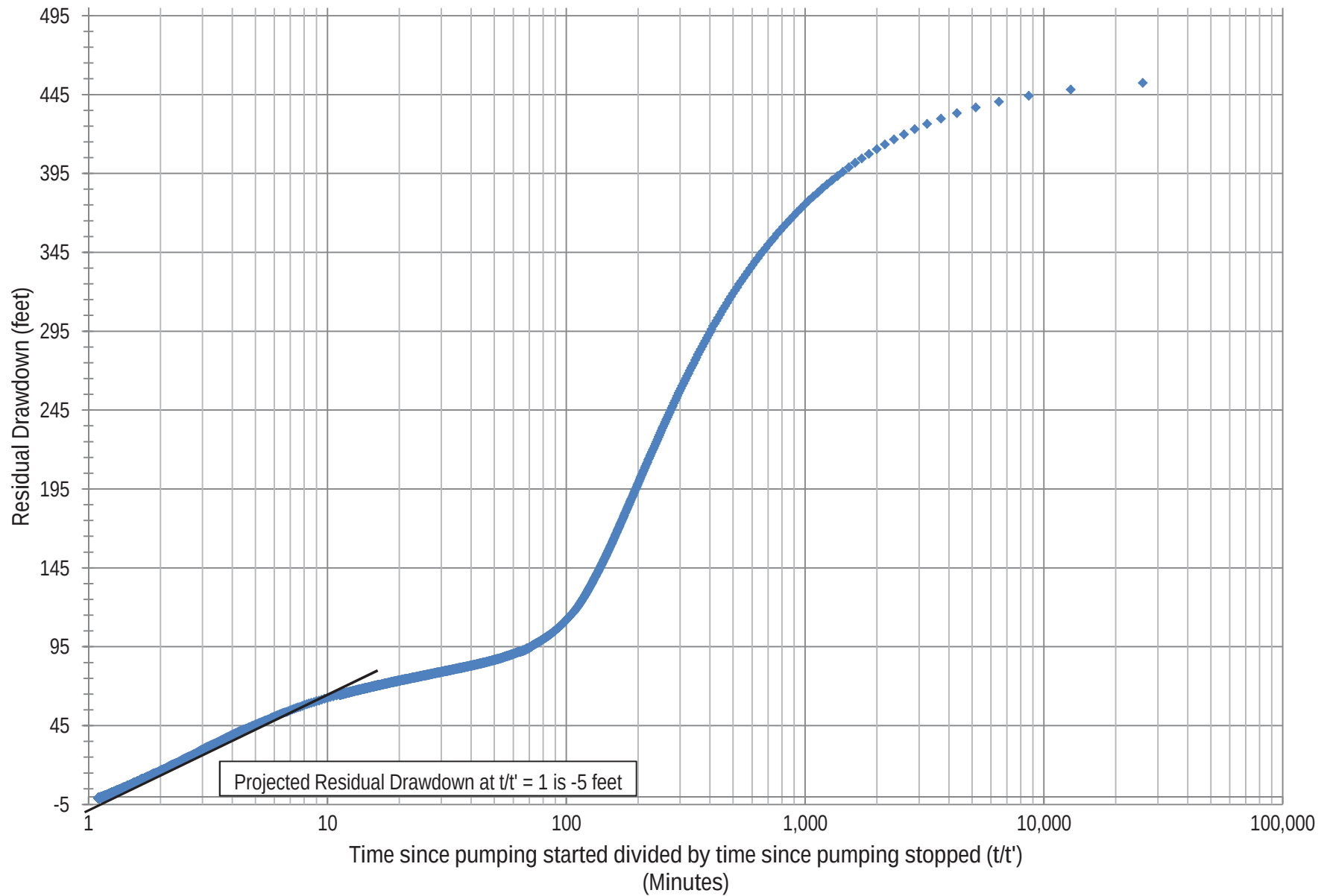
Figure 34. Onsite Well B Constant Rate Test Recovery Analysis
