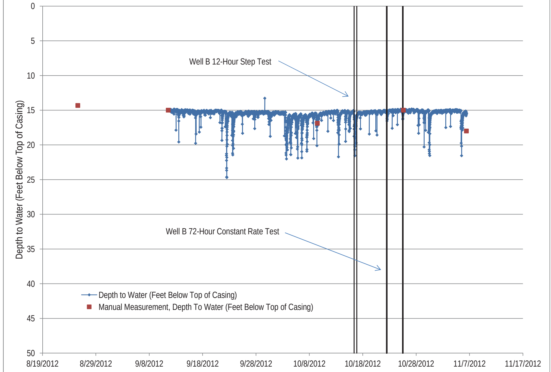
Figure 26. Off-site Well RSH-1 Water Level Data
