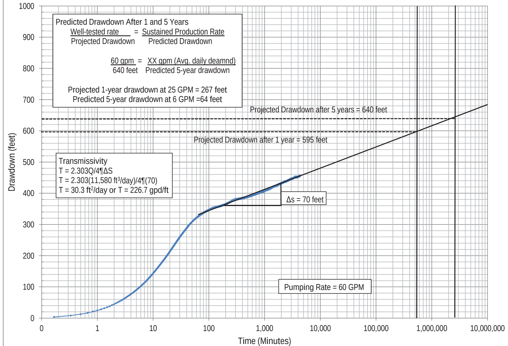
Figure 33. Onsite Well B Constant Rate Test Jacob Straight Line Analysis
