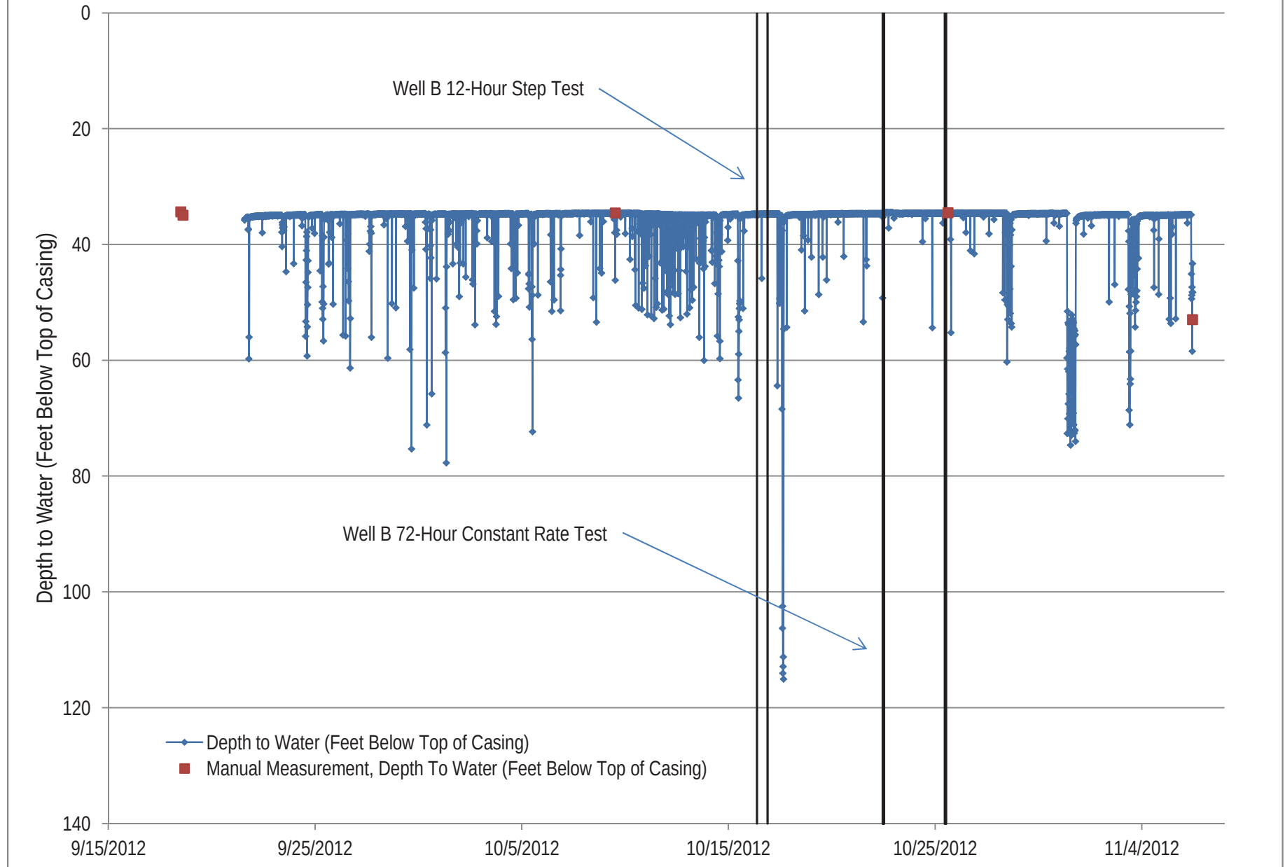
Figure 25. Off-site Well RSD-1 Water Level Data
