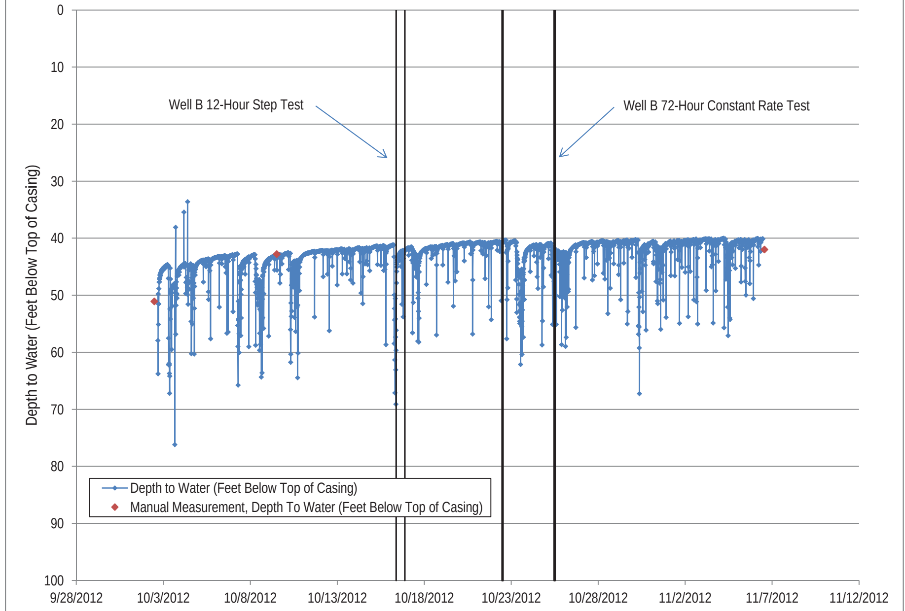
Figure 29. Off-site Well WHH-1 Water Level Data
