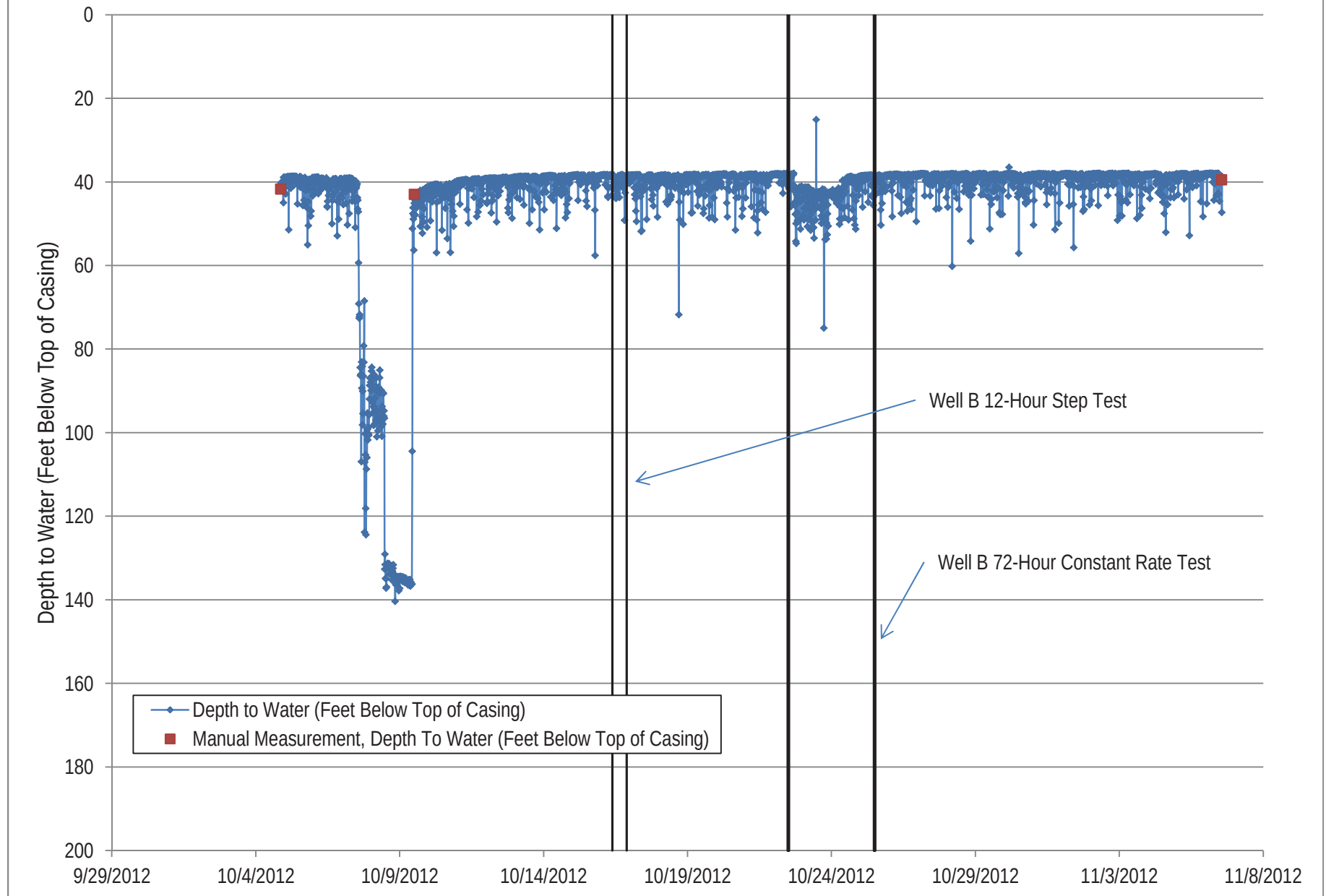
Figure 21. Off-site Well GS-2 Water Level Data
