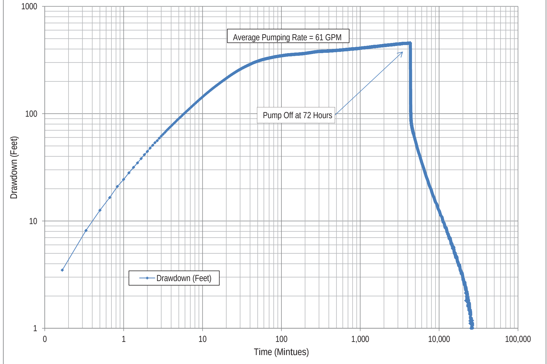
Figure 32. Onsite Well B Constant Rate Test Log Water Level Drawdown
