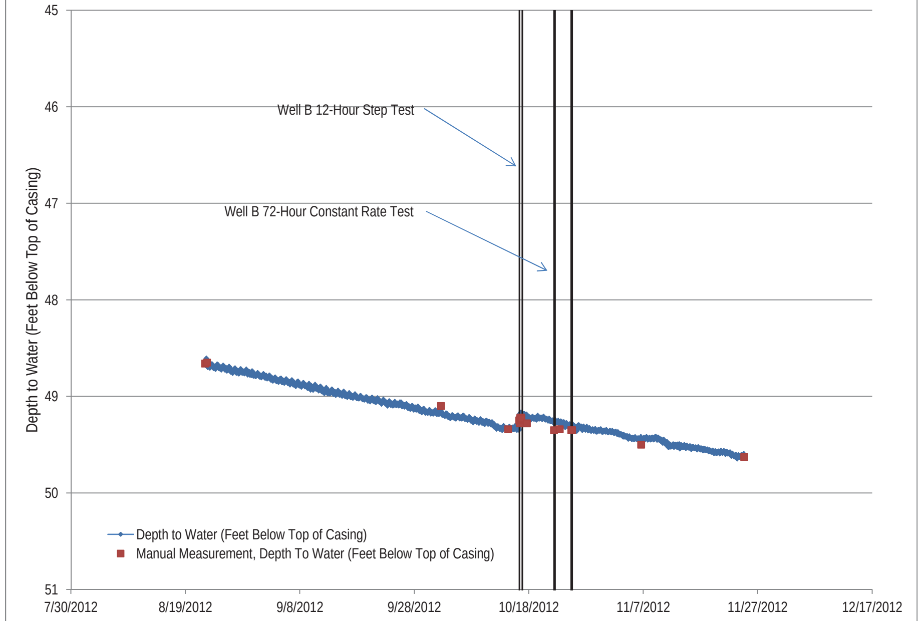
Figure 17. On-site Well A Water Level Data
