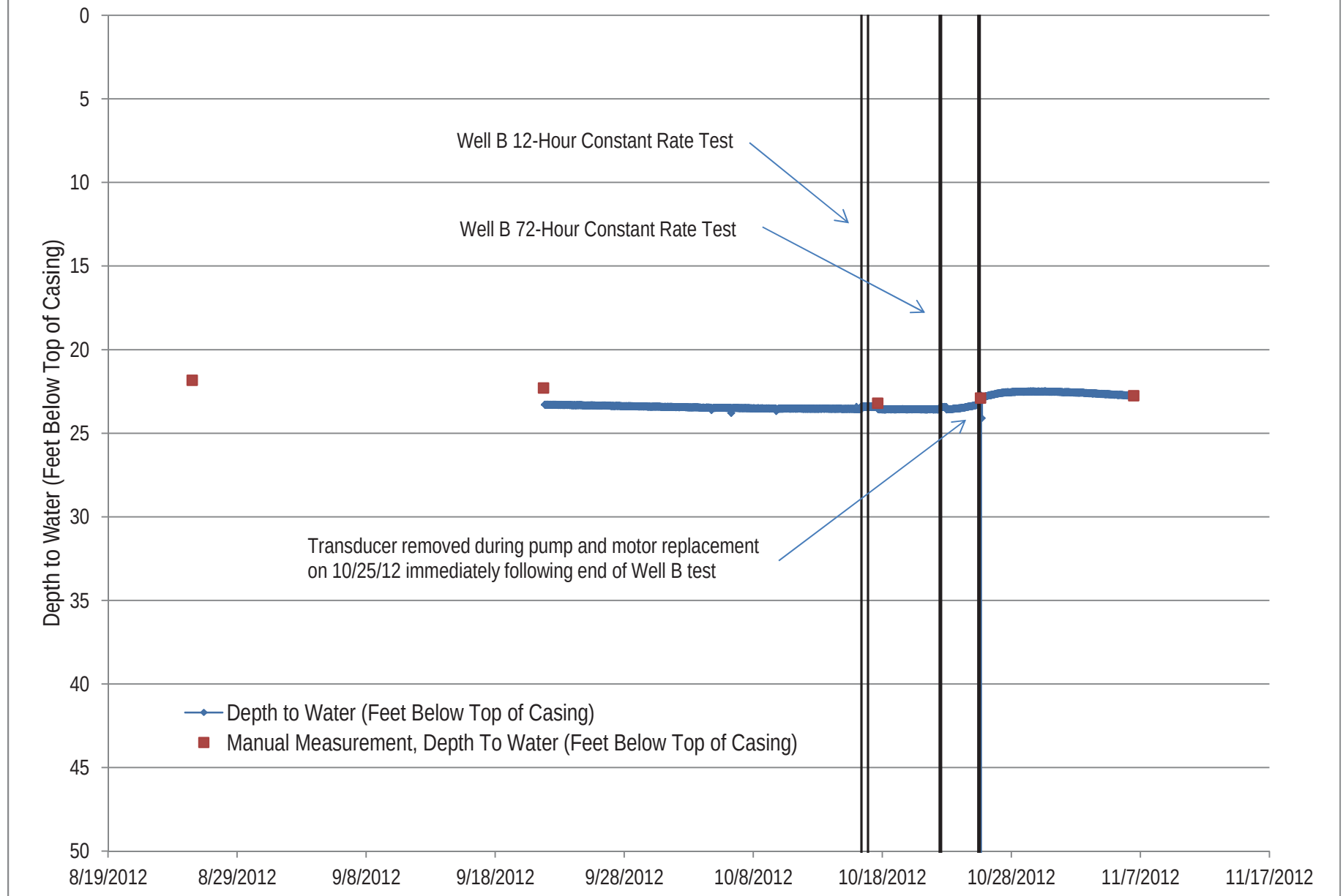
Figure 24. Off-site Well RM-3 Water Level Data
