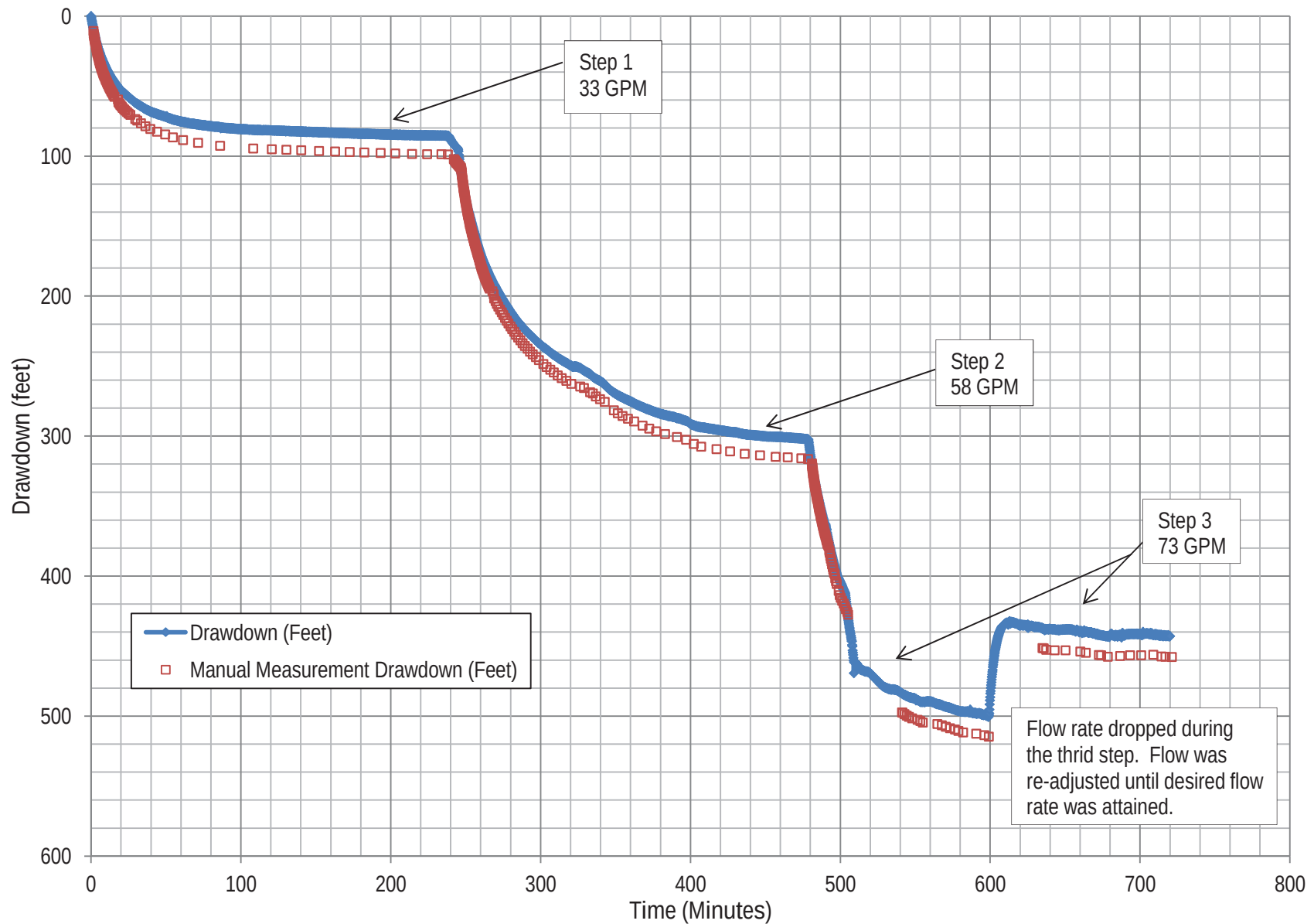
Figure 30. Onsite Well B Step Test Water Level Drawdown
