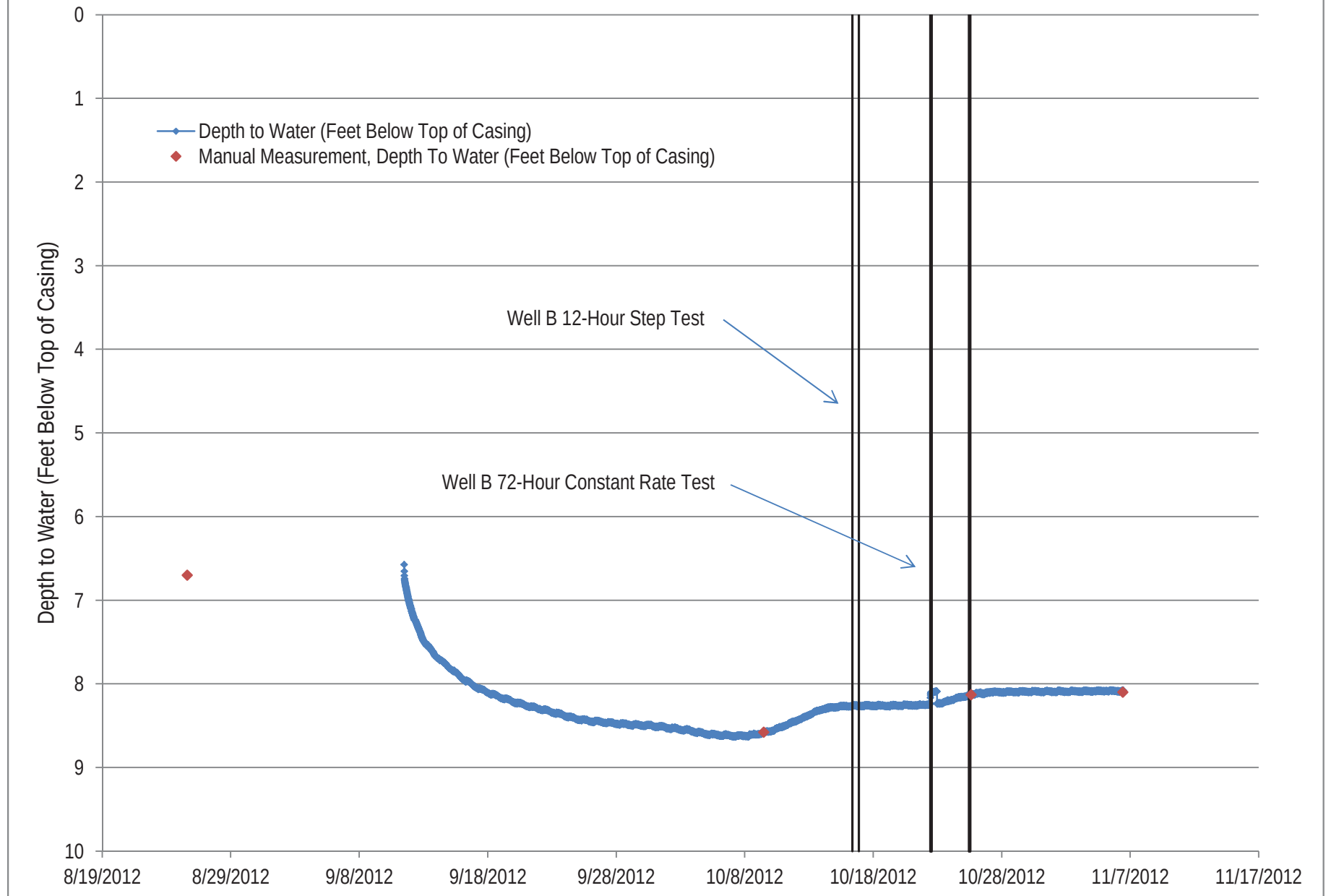
Figure 27. Off-site Well RSH-2 Water Level Data
