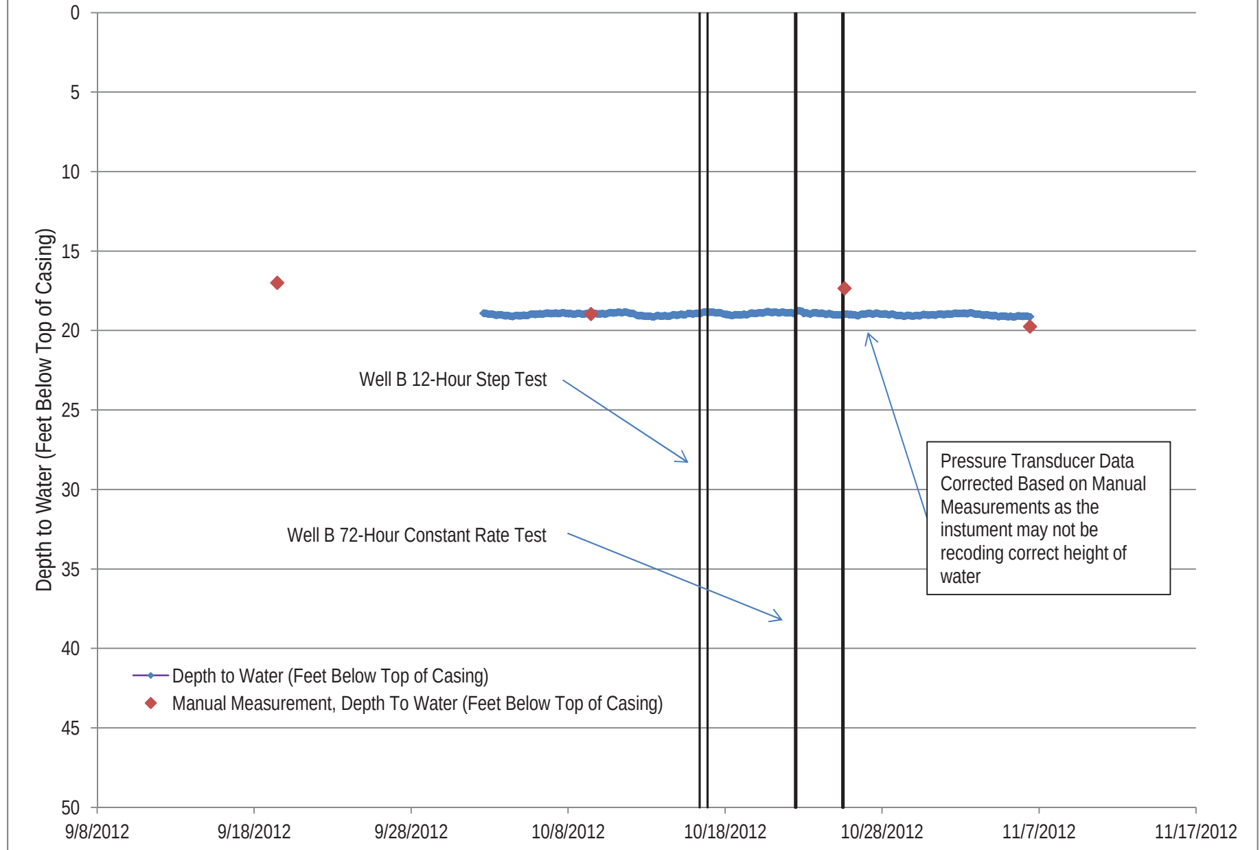
Figure 28. Off-site Well RSH-3 Water Level Data
