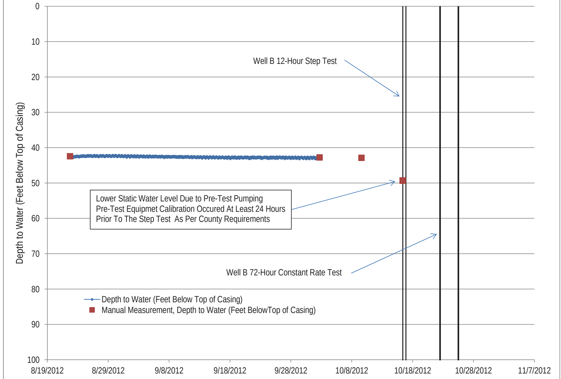
Figure 18. On-site Well B Pre-Test Water Level Data
