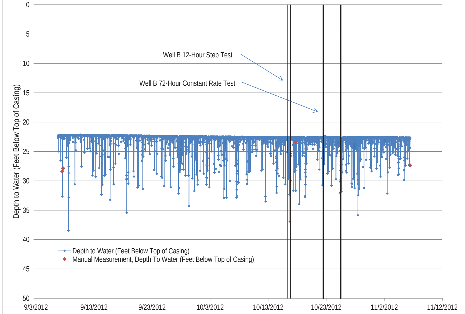
Figure 23. Off-site Well RM-1 Water Level Data
