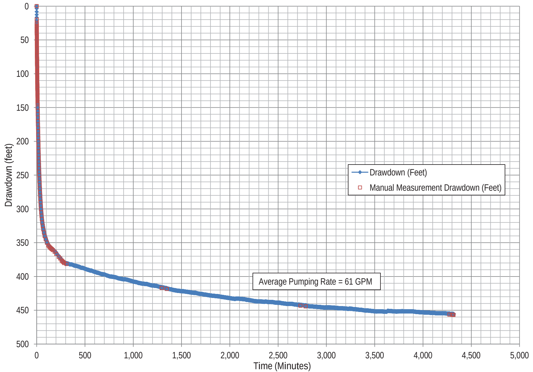
Figure 31. Onsite Well B Constant Rate Test Water Level Drawdown
