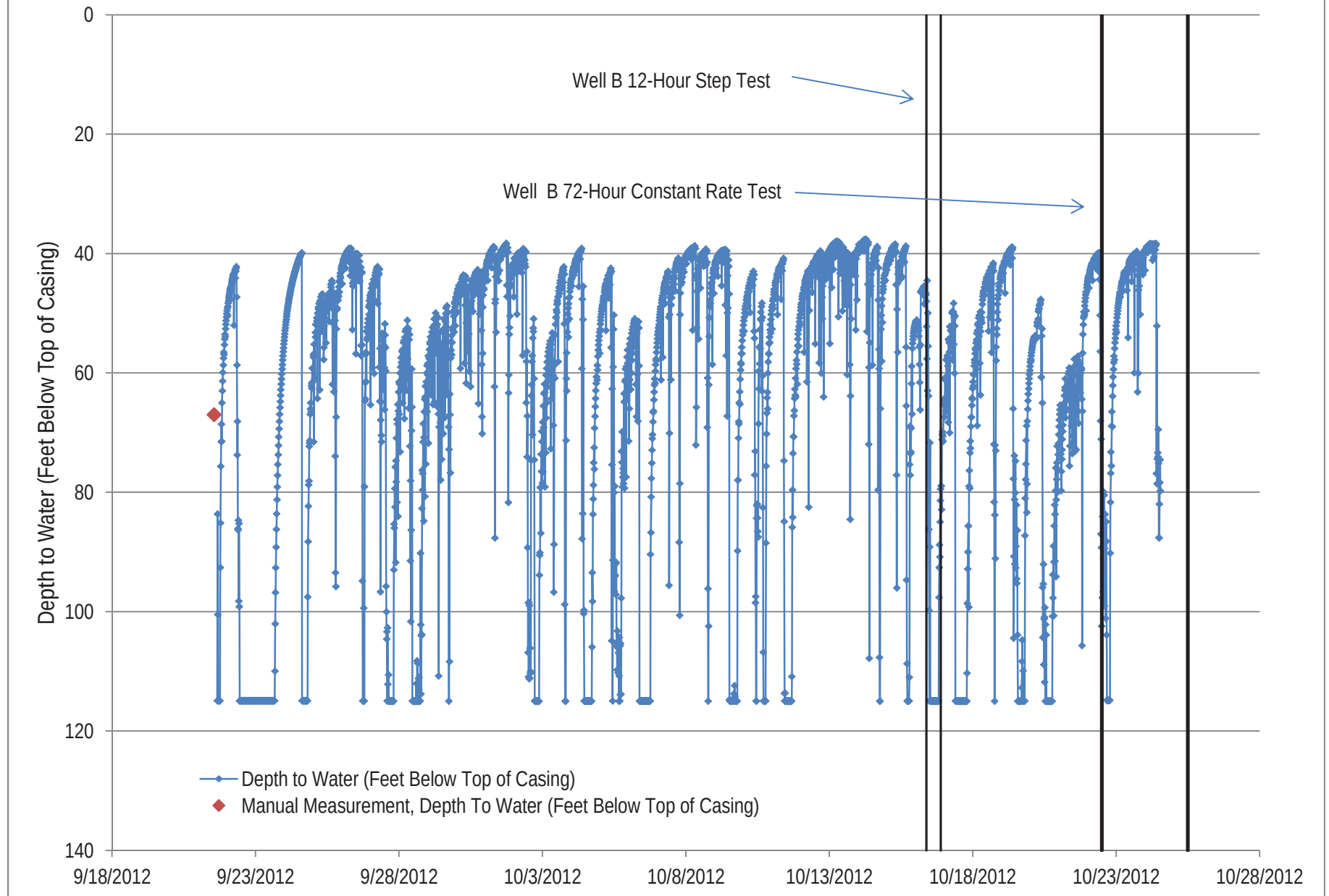
Figure 19. Off-site Well GR-1 Water Level Data
