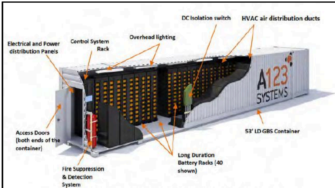
Figure 4: Example Battery Storage Container
