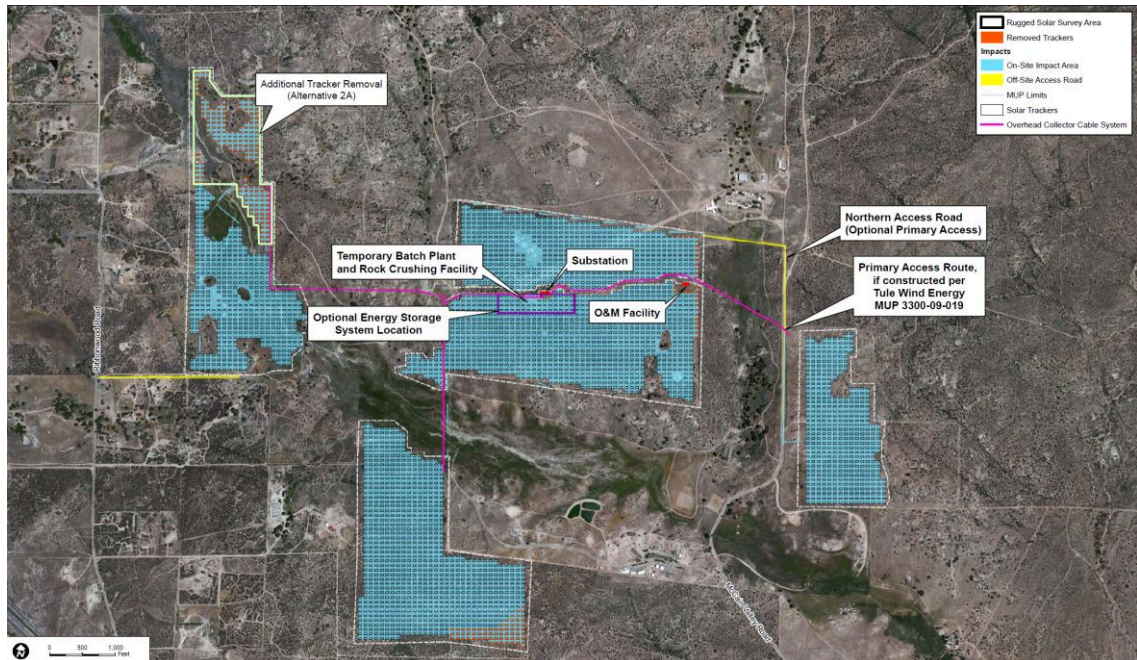
Figure 3: Rugged Solar Project Layout- Alternative 2A
