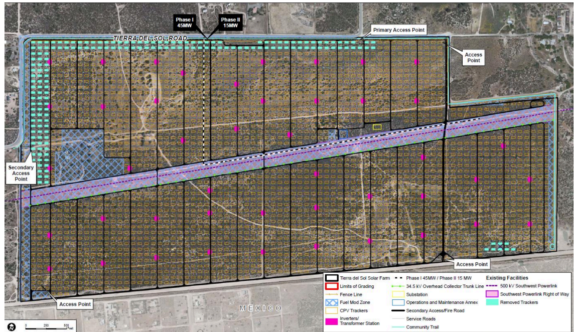
Figure 6: Tierra Del Sol Solar Project Layout- Alternative 2
