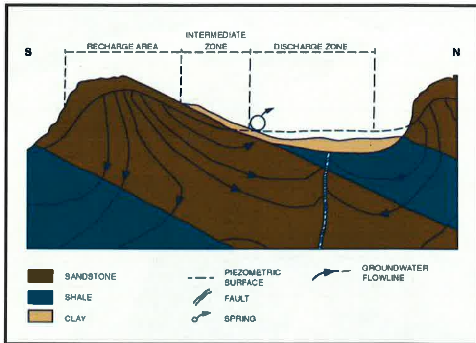
Fig. 5 Typical location of recharge and discharge of groundwater.
