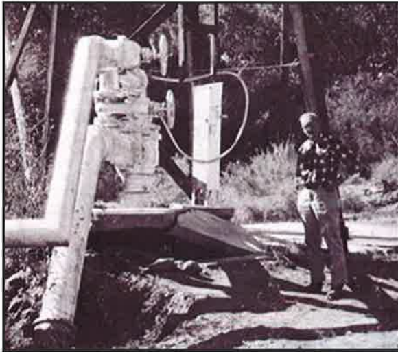
Fig. 28 Timed photographs of a protruding well in Las Vegas, Nevada, showing evidence of land subsidence (From Pavelko et al. : Las Vegas, Nevada , in U.S. Geological Survey Circular 1182).
