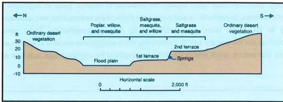
Fig. 11 Vegetational gradient along a cross section of the Mohave river valley at Camp Cadiz, California.
