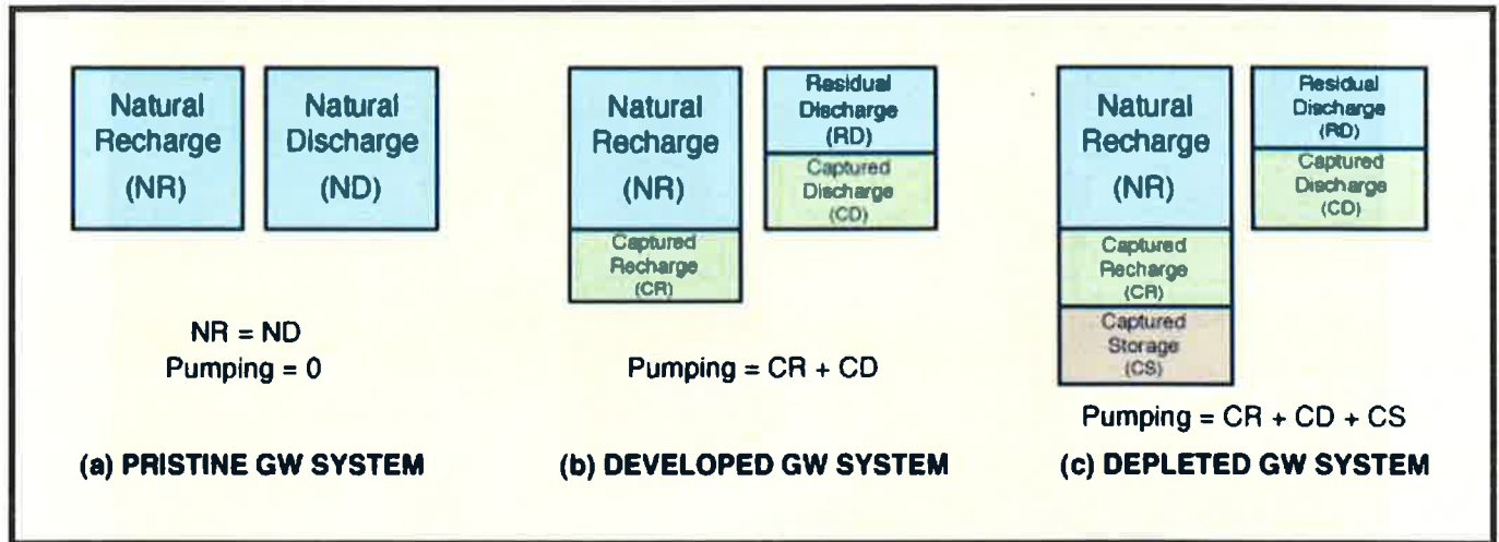
Fig. 32 Stages in the development of groundwater systems.
