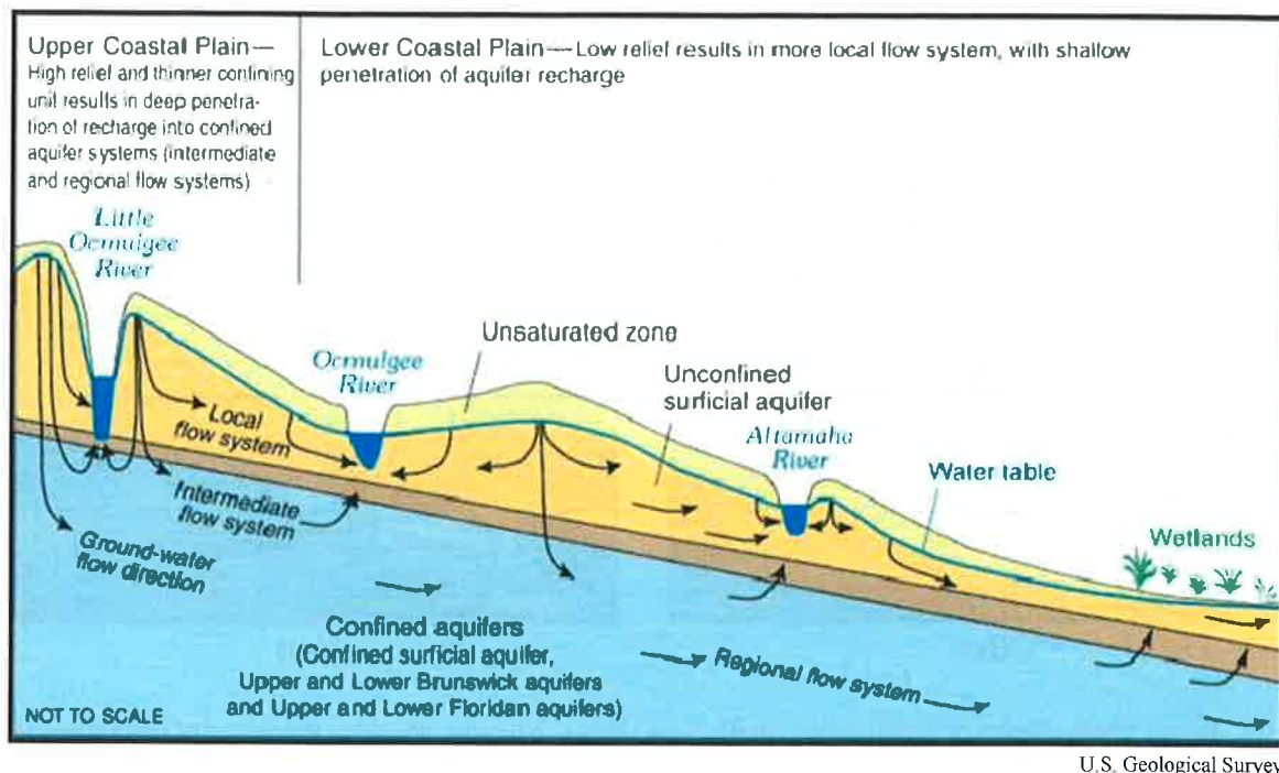
Fig. 29 Conceptual hydrological flow system in the coastal plains of Georgia.
