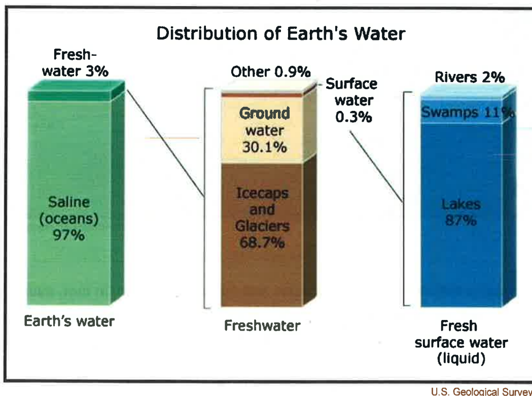
Fig. 3 Distribution of Earth's water.
