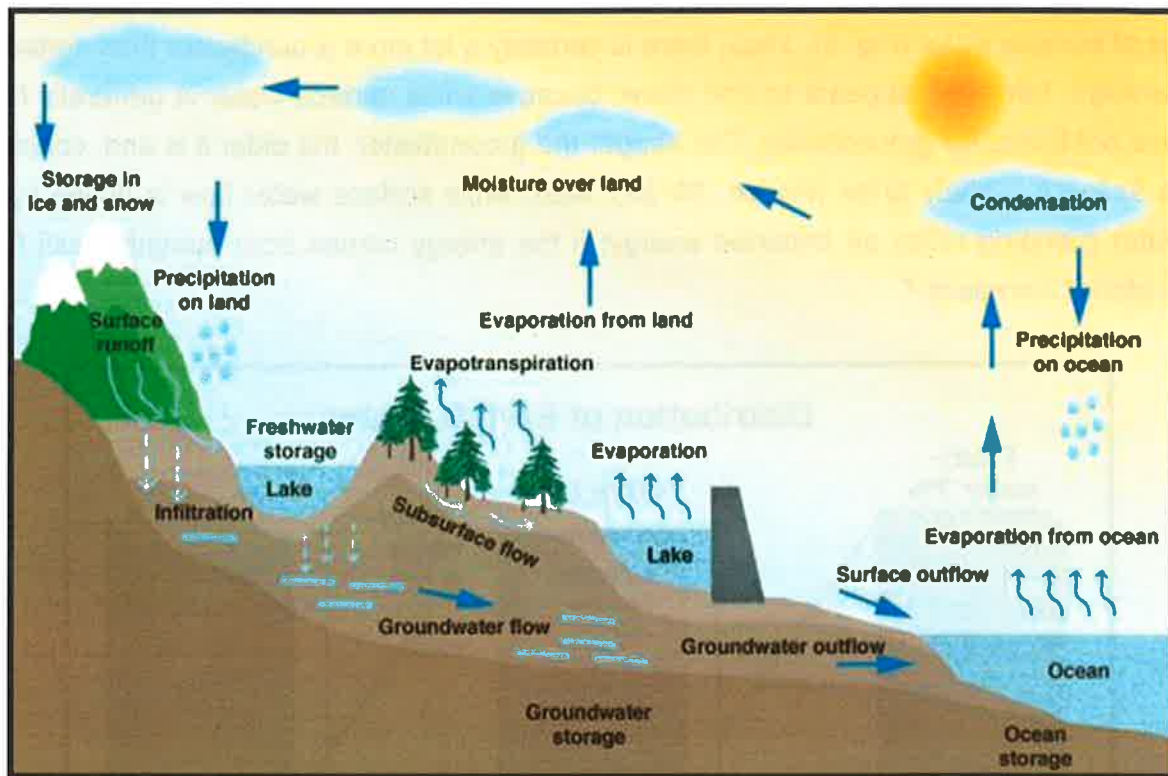
Fig. 2 The hydrologic cycle.
