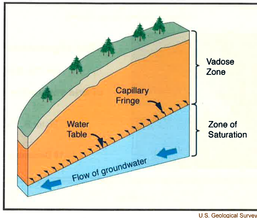
Fig. 1 Vadose zone and zone of saturation in subsurface flow.
