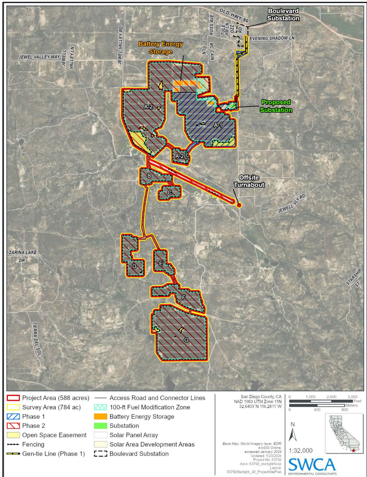
Figure A2. Starlight Solar Energy Storage Project site plan.
