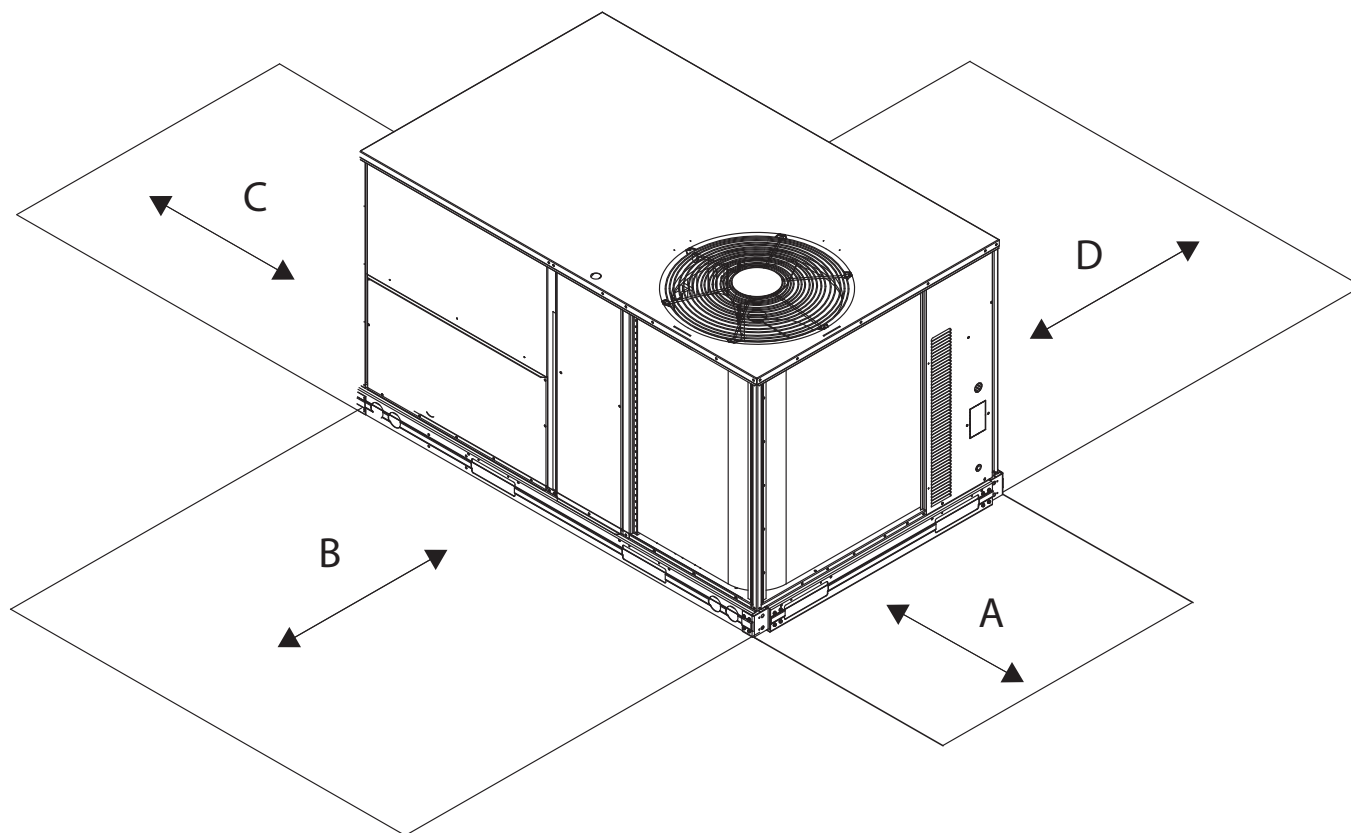
SERVICE CLEARANCE DIMENSIONAL DRAWING - UNIT SIZES 04-06
