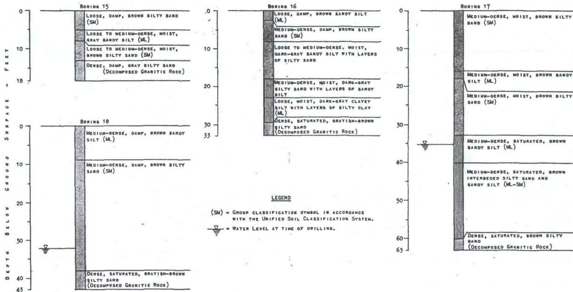
LOGS OF TEST BORINGS 15 THRU 18 PINE VALLEY BASIN JOB NO. 61-245
