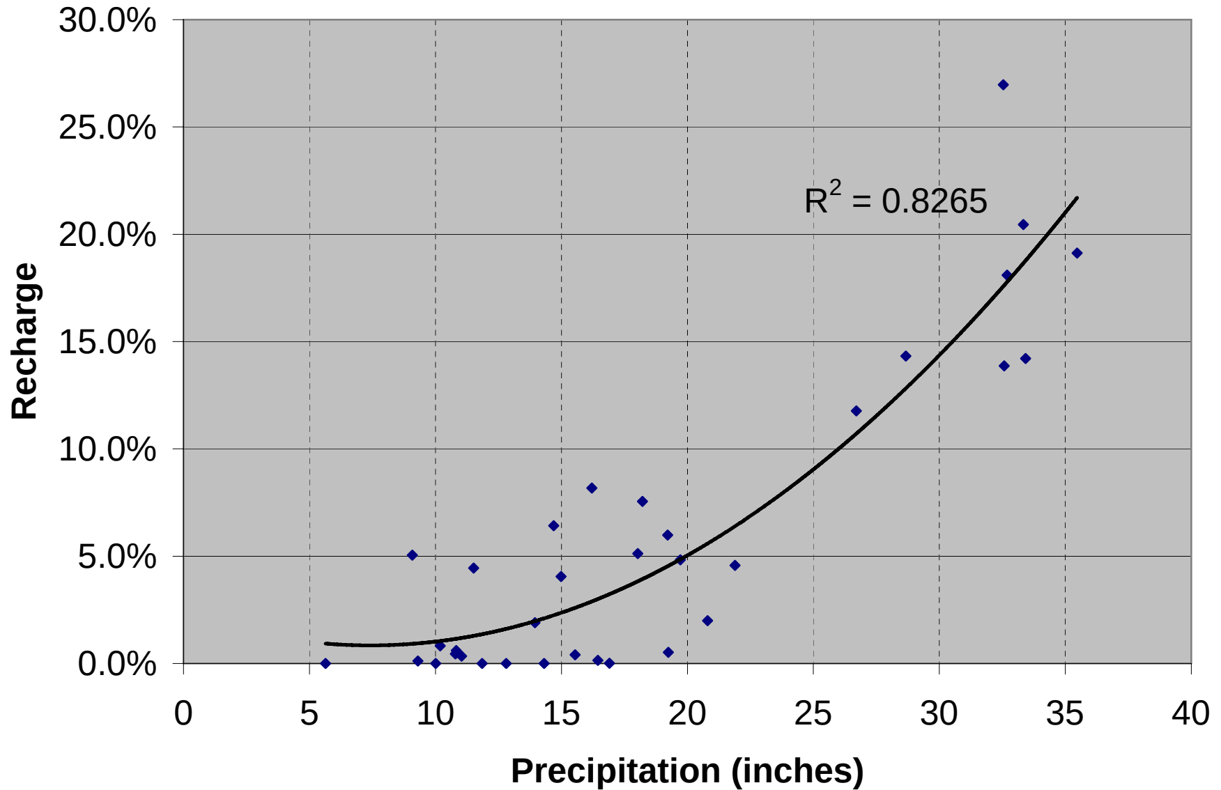
Figure D-4: Recharge Efficiency - Calibrated Lee Valley Results
