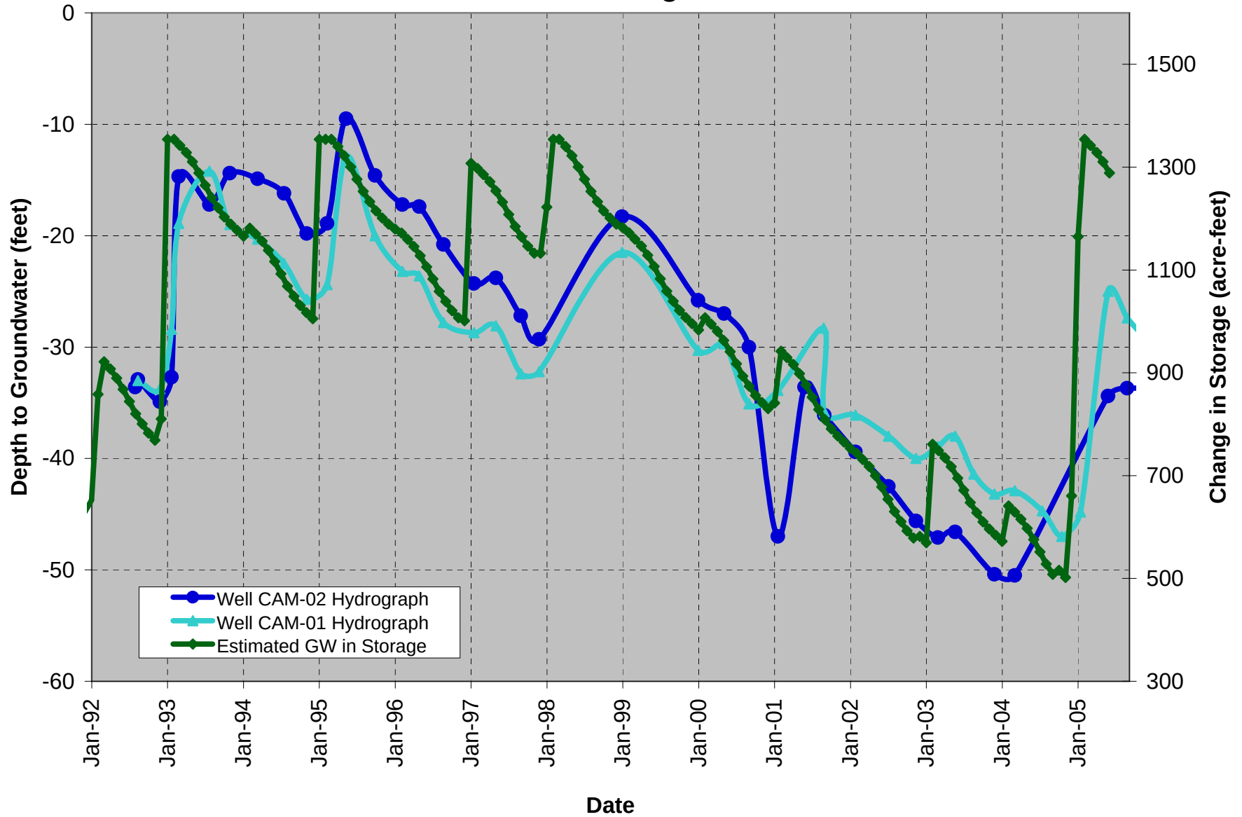
Figure D-10 Morena South Basin Estimated Groundwater in Storage vs. Groundwater Levels
