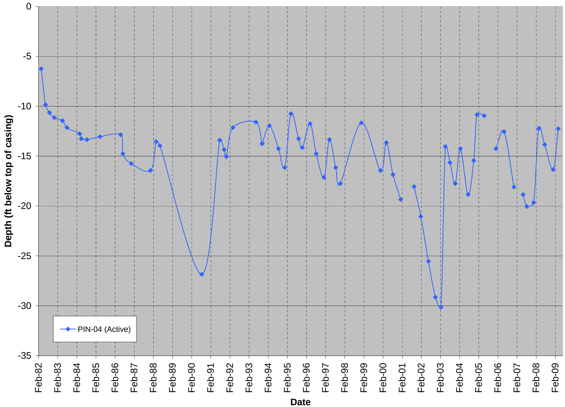
Figure 16: Pine Valley Area 5 Well Hydrographs
