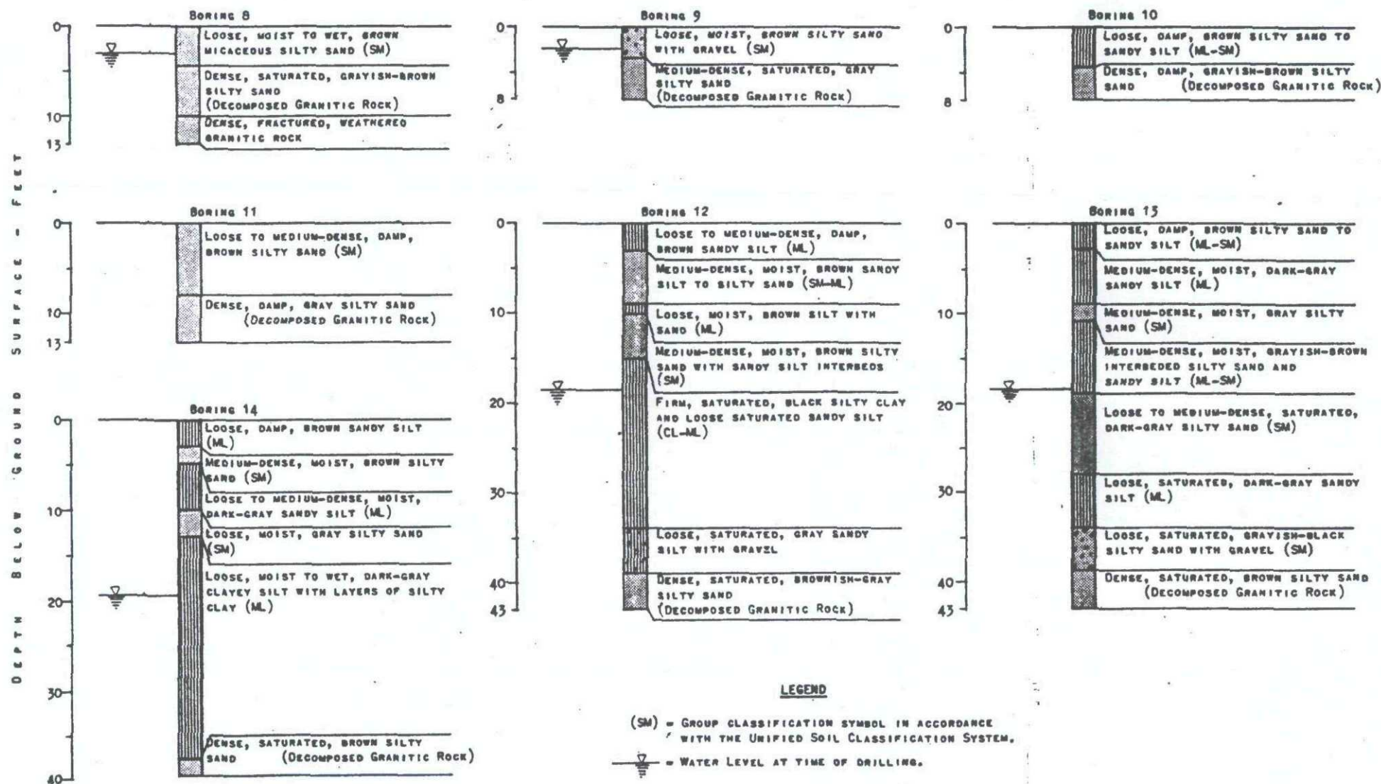
LOGS OF TEST BORINGS 8 THRU 14 PINE VALLEY BASIN JOB NO. 61-245
