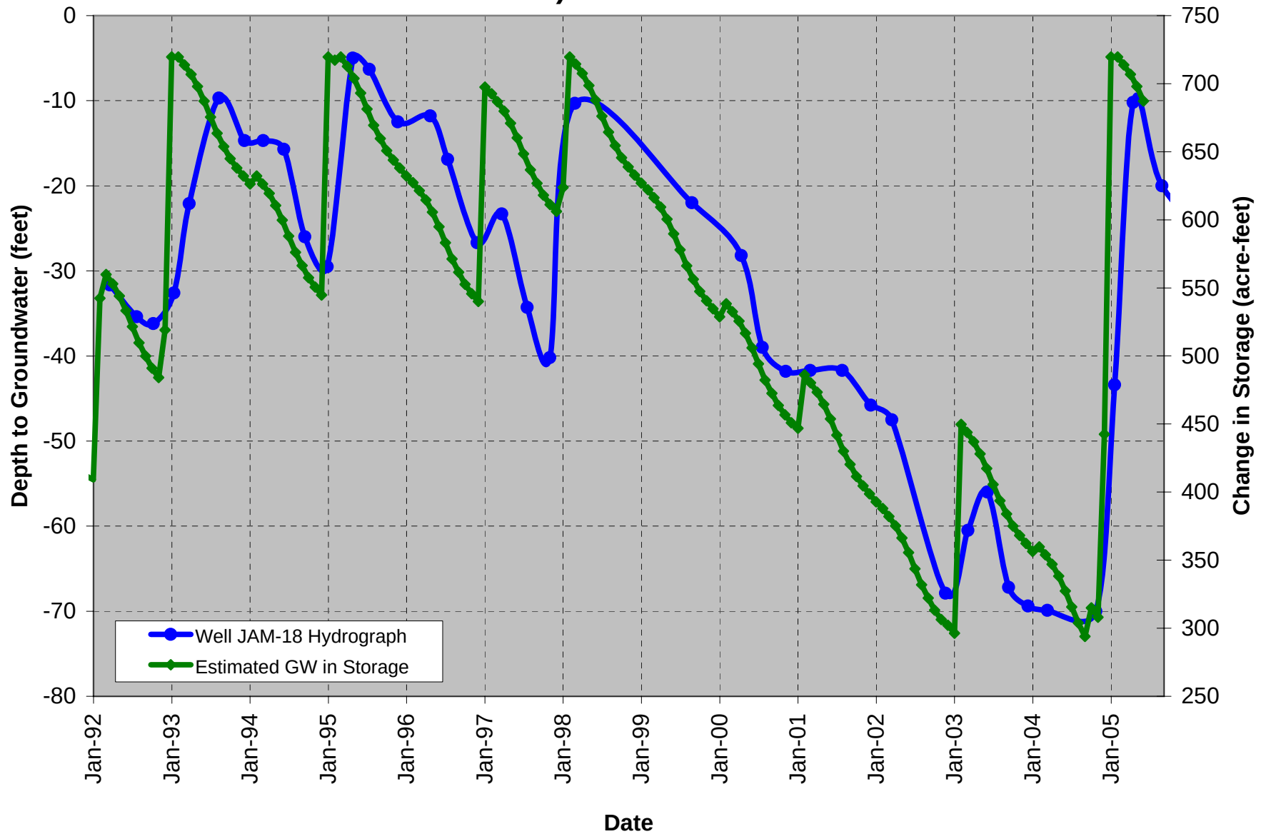
Figure D-3 Lee Valley –Estimated Groundwater in Storage (50% of Runoff Calculated) vs. Groundwater Levels
