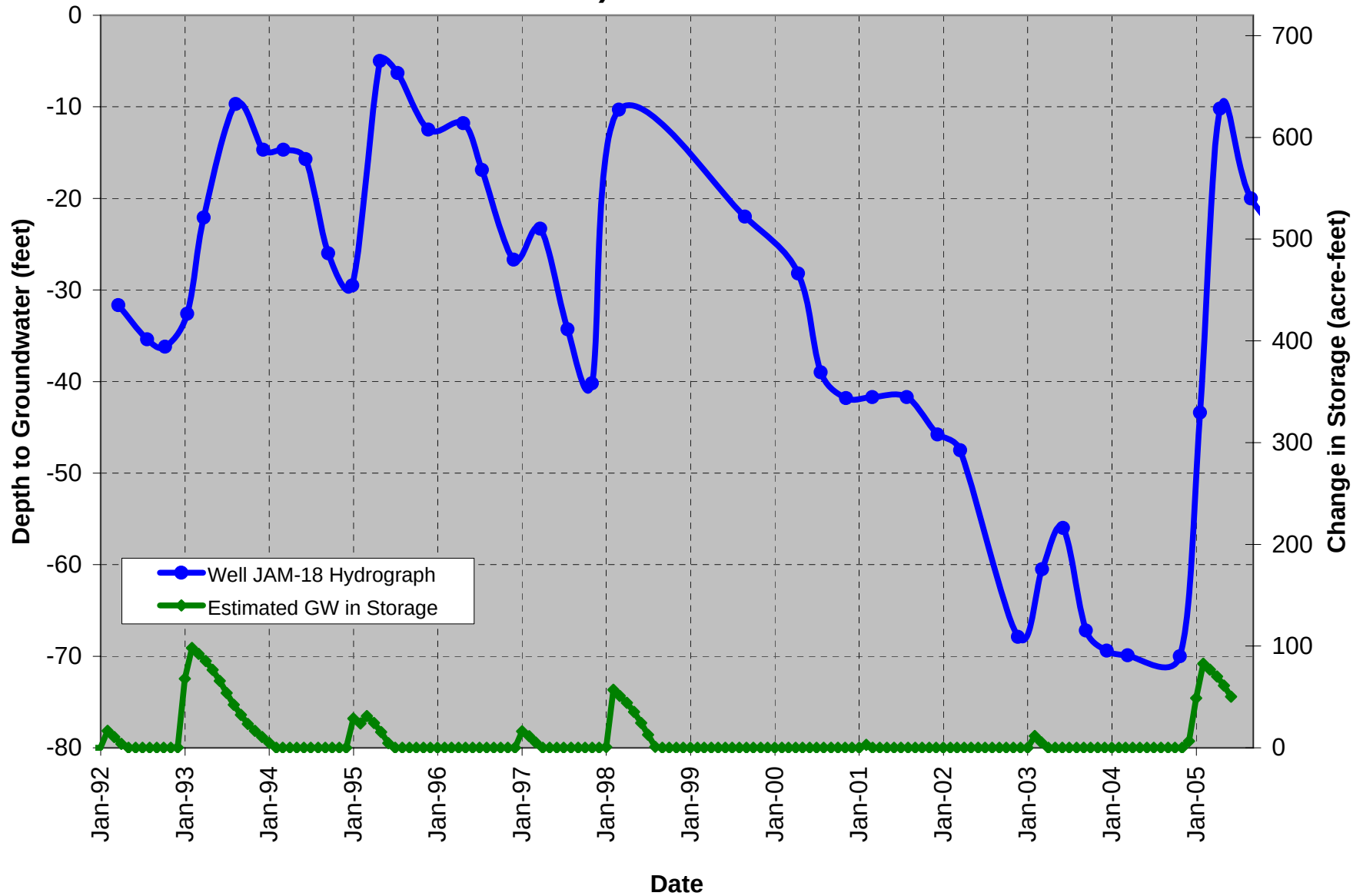
Figure D-2 Lee Valley –Estimated Groundwater in Storage (100% of Runoff Calculated) vs. Groundwater Levels
