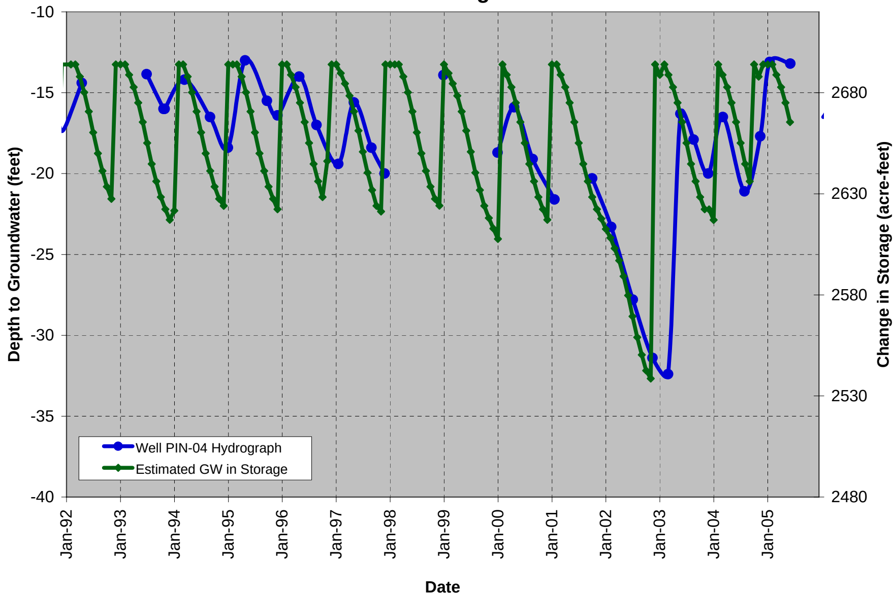
Figure D-7 Pine North Basin Estimated Groundwater in Storage vs. Groundwater Levels
