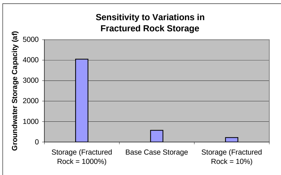
Figure D-12 Sensitivity Analysis Groundwater in Storage and Groundwater Demand
