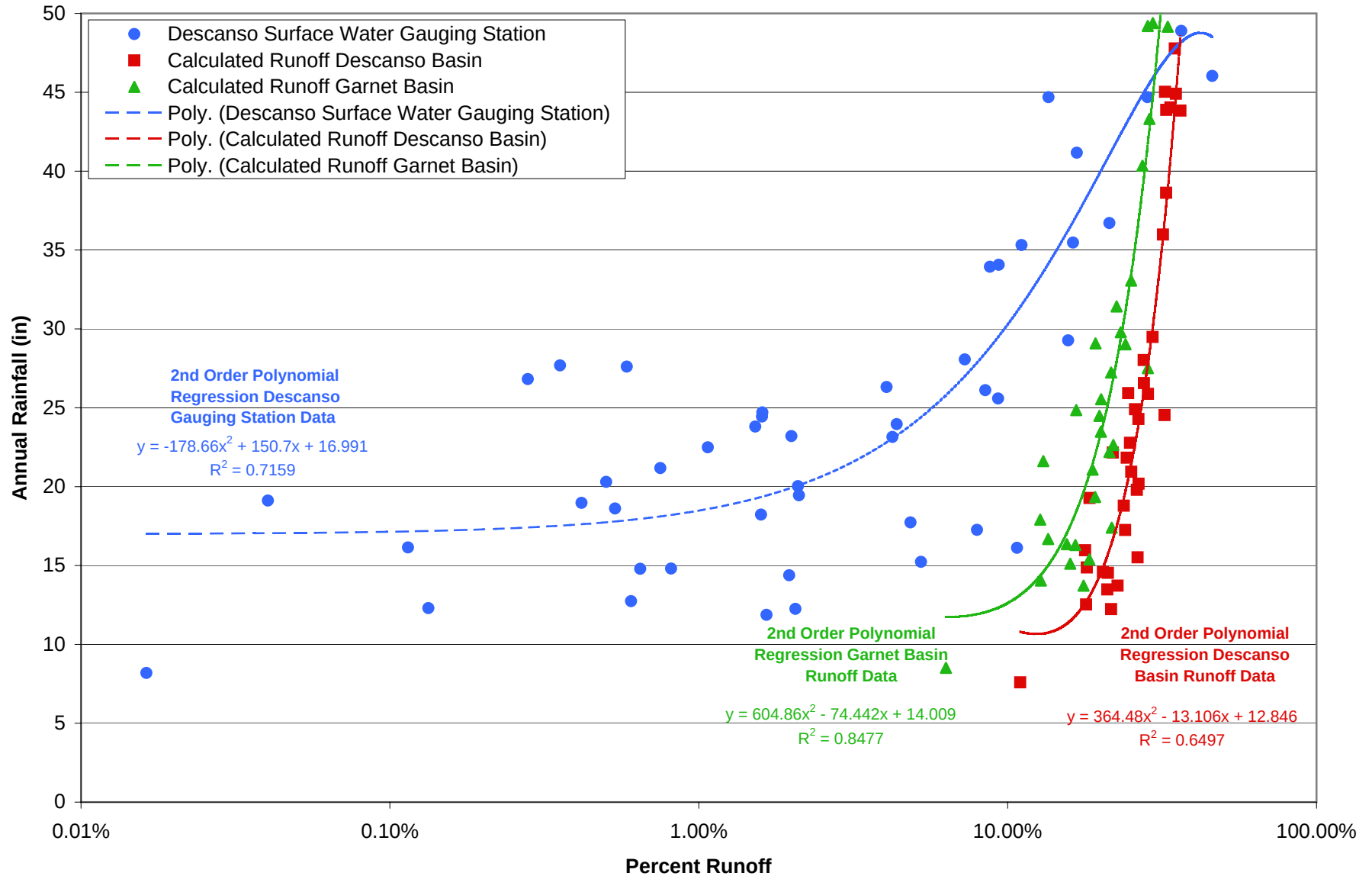
FIGURE D-5 Annual Rainfall vs Percent of Runoff Descanso Gauging Station and Calculated Runoff For Descanso and Garnet Basins
