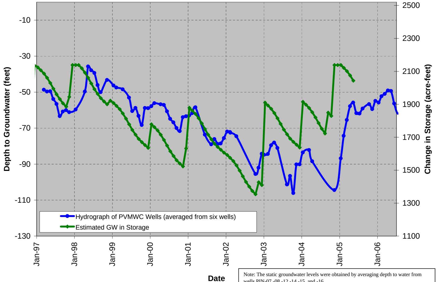
Figure D-8 Pine South Basin Estimated Groundwater in Storage vs. Groundwater Levels
