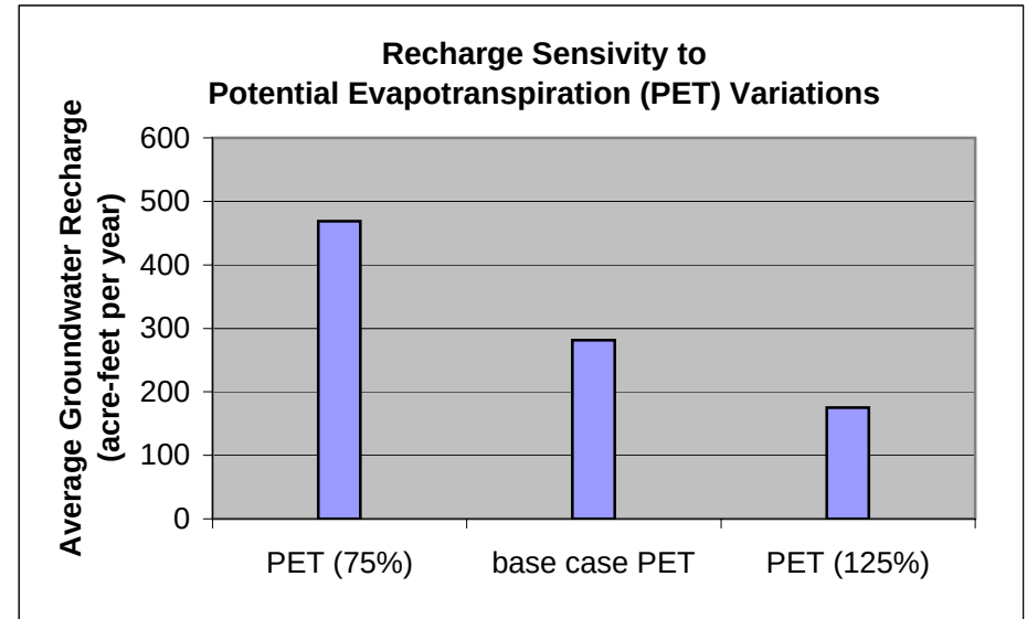
Figure D-11 Sensitivity Analysis - Groundwater Recharge Parameters
