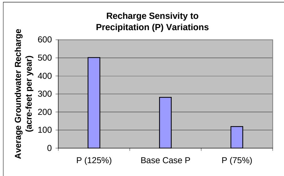
Figure D-11 Sensitivity Analysis - Groundwater Recharge Parameters
