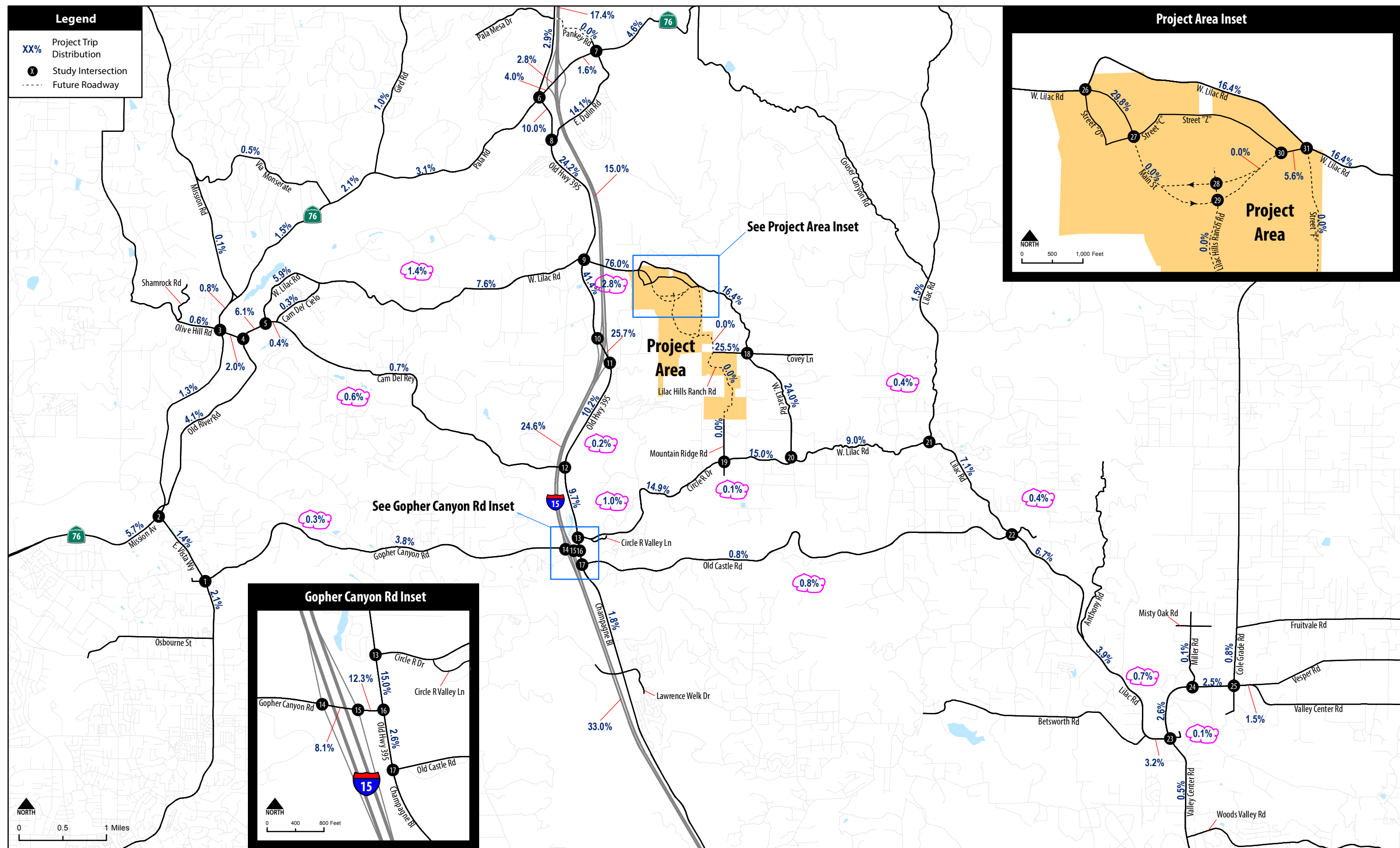
Figure 4-4 Project Trip Distribution (Phase B) - Existing Network
