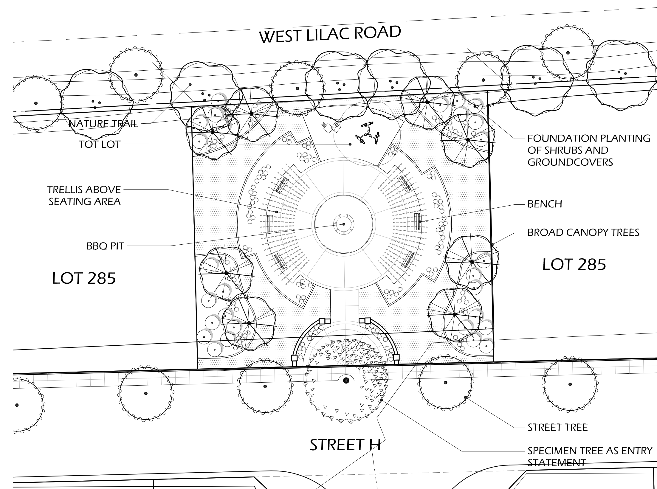
PARK P5 - NEIGHBORHOOD PARK
