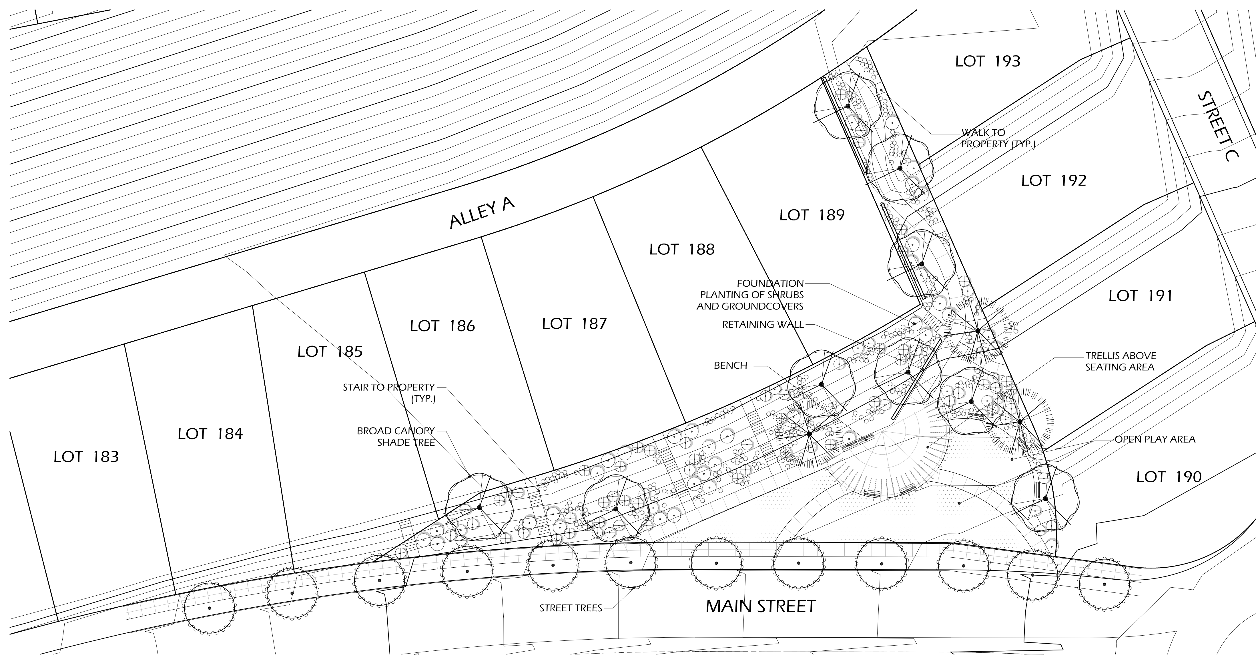
PARK P3 - Garden Park
