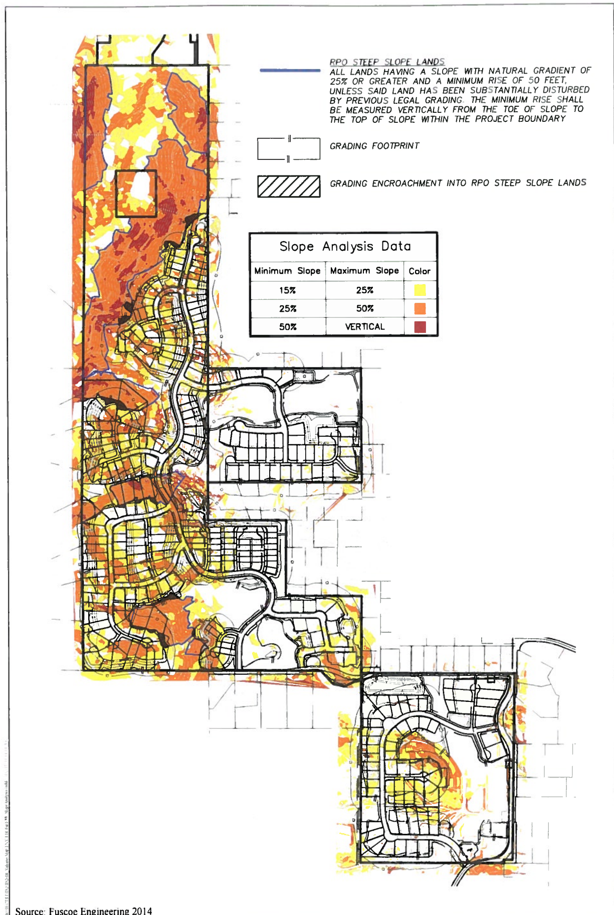
Site Topography/Slope Analysis
