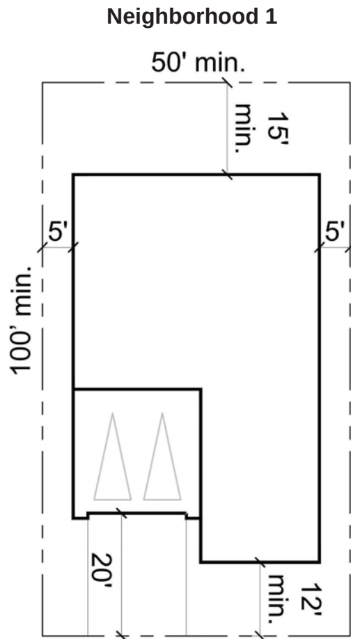
Neighborhood 1 Courtyard Configuration
