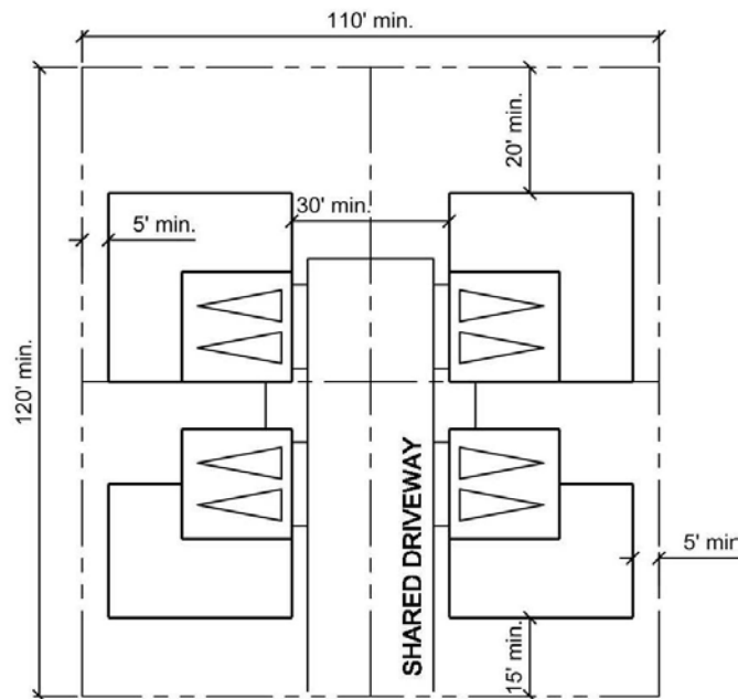
Neighborhood 1 Courtyard Configuration
