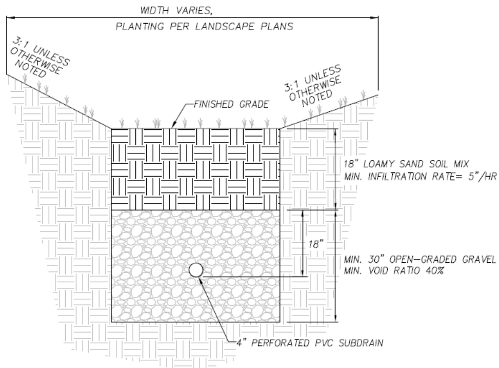
TYPICAL DETAIL - BIORETENTION BASIN
