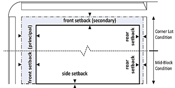
C. OUTBUILDING PLACEMENT DIAGRAM
