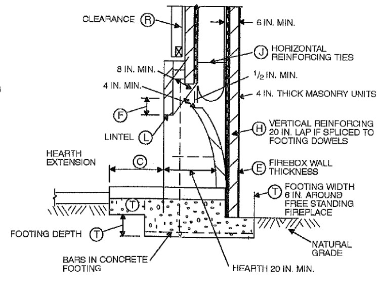
BRICK FIREBOX AND CHIMNEY ON CONCRETE SLAB
