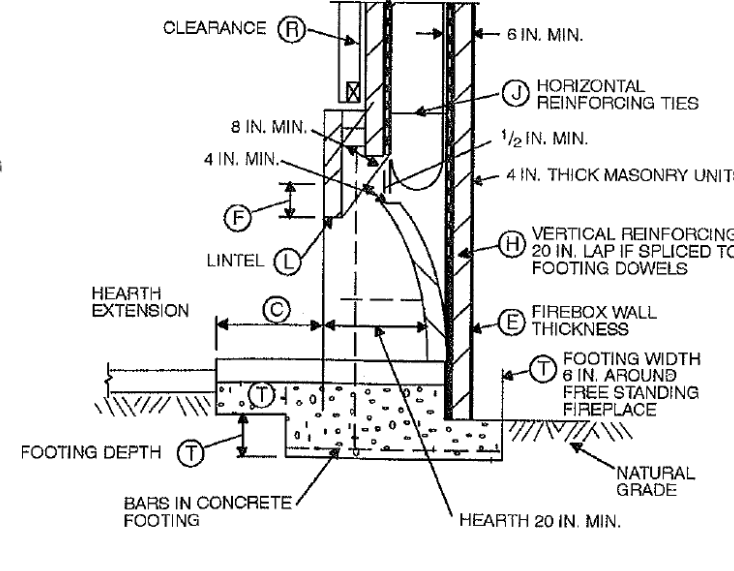
BRICK FIREBOX AND CHIMNEY ON CONCRETE SLAB
