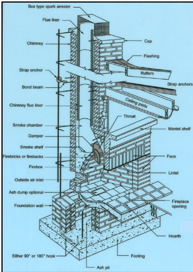
PARTS OF A FIREPLACE AND CHIMNEY
