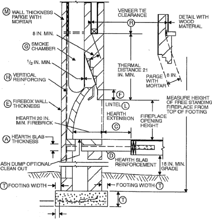
BRICK FIREBOX AND CHIMNEY WITH WOOD FLOORS
